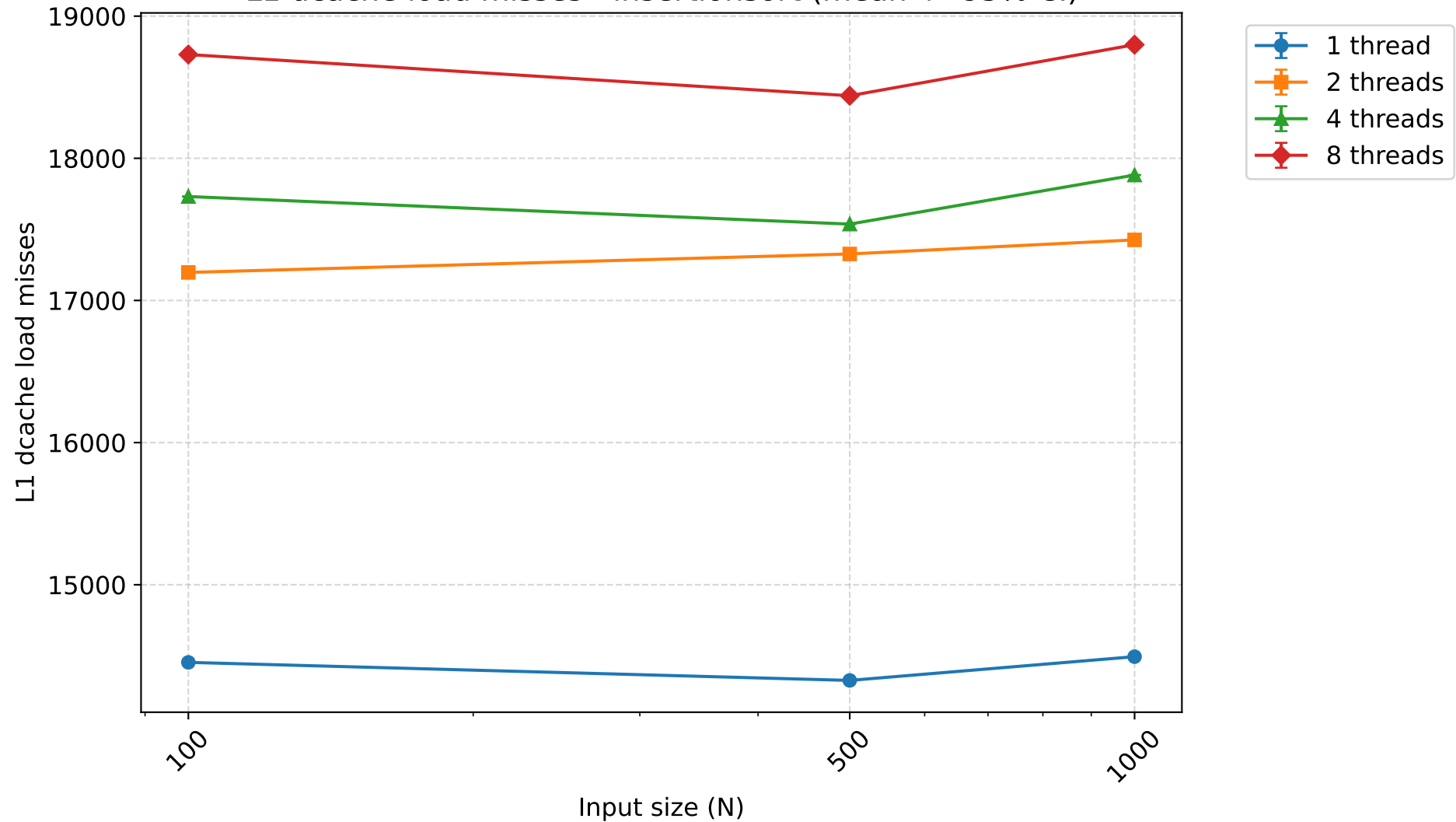
L1 dcache load misses - insertionsort (mean \pm 95% CI)
