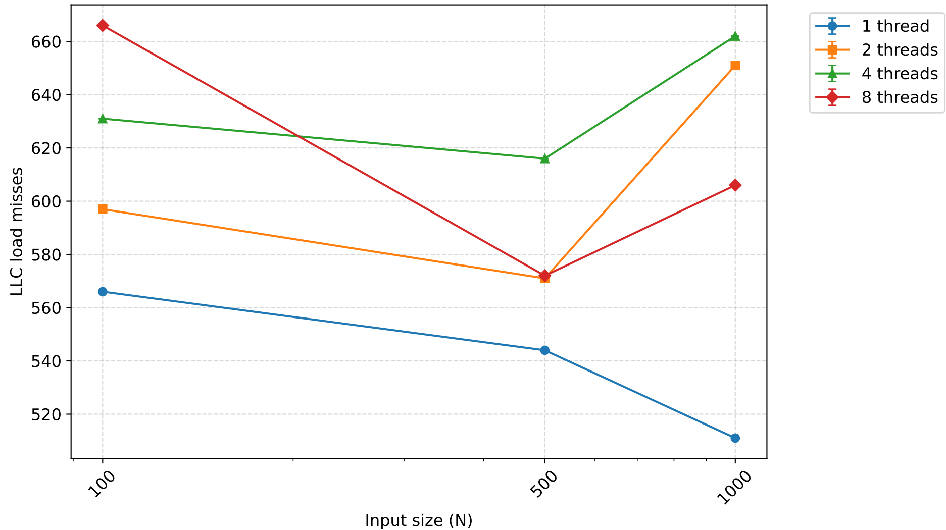
LLC load misses - insertionsort (mean \pm 95% CI)
