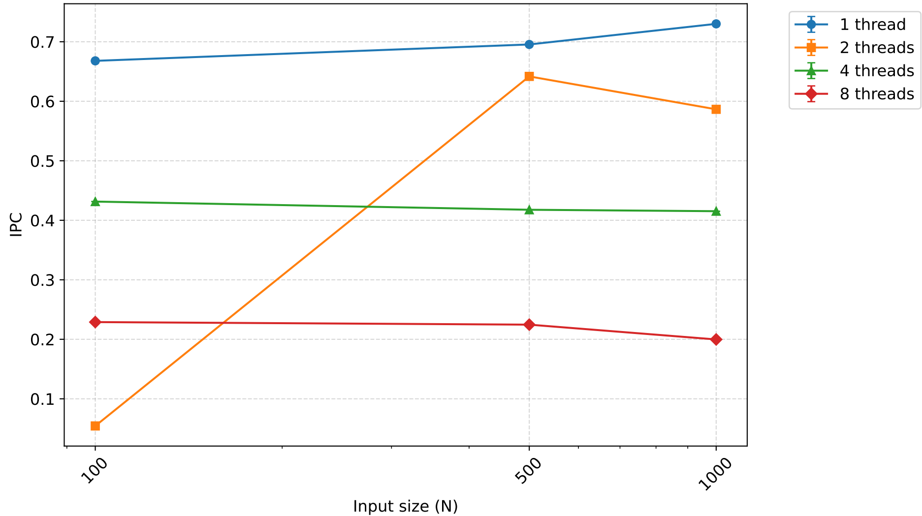
IPC - insertionsort (mean \pm 95% CI)
