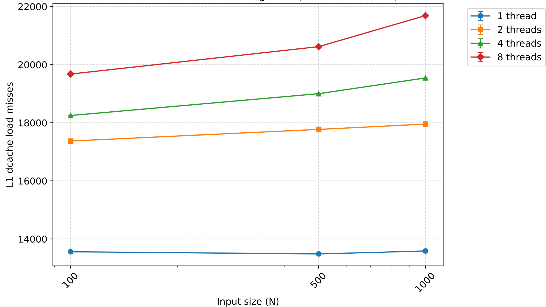
L1 dcache load misses - mergesort (mean \pm 95% CI)
