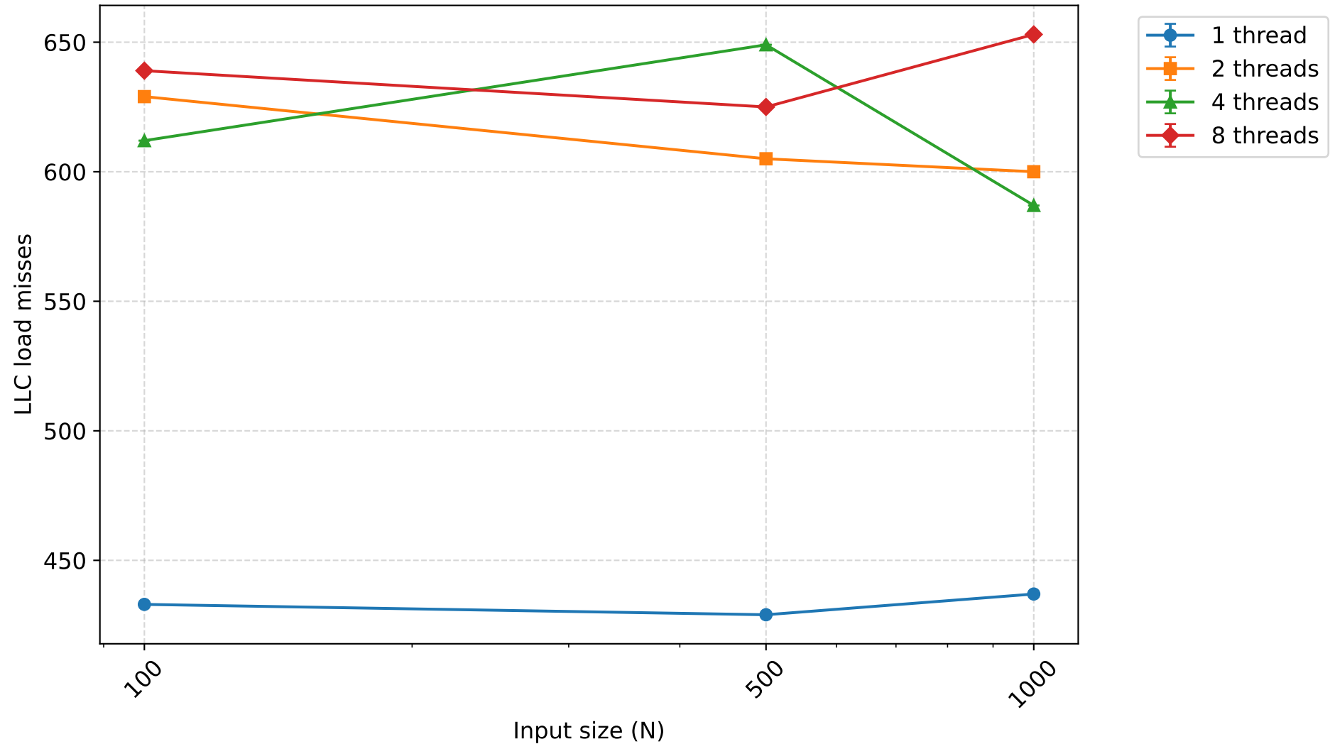
LLC load misses - mergesort (mean \pm 95% CI)
