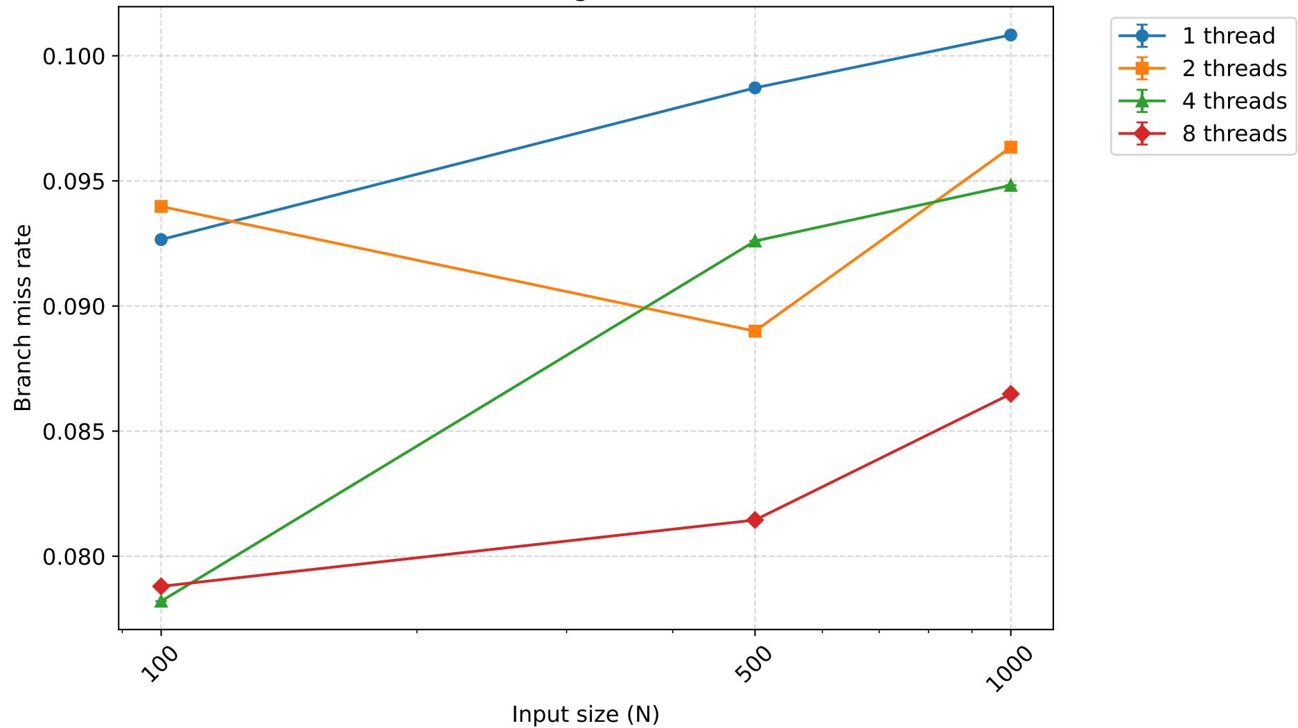
Branch miss rate - mergesort (mean \pm 95% CI)
