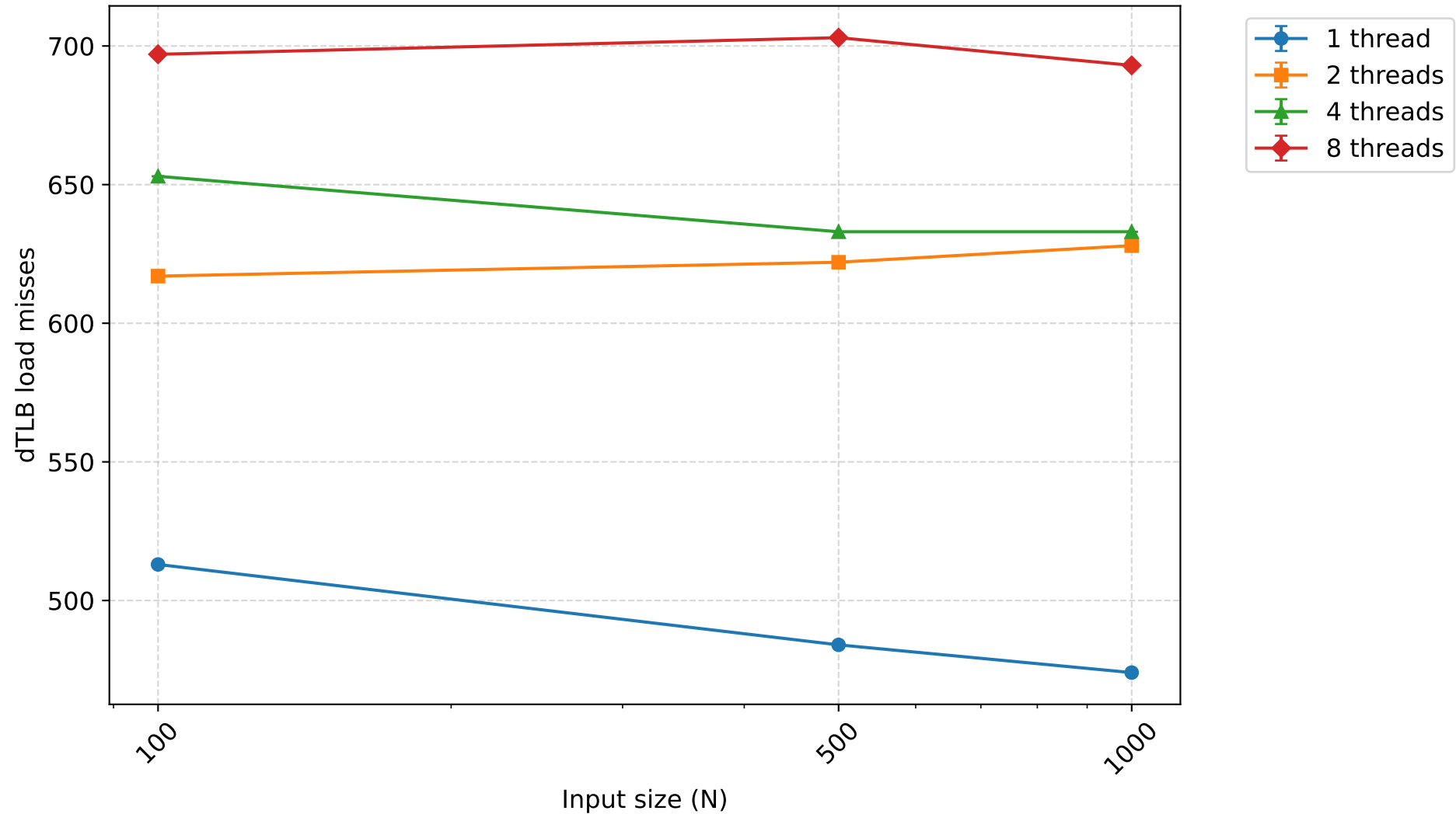
dTLB load misses - mergesort (mean \pm 95% CI)
