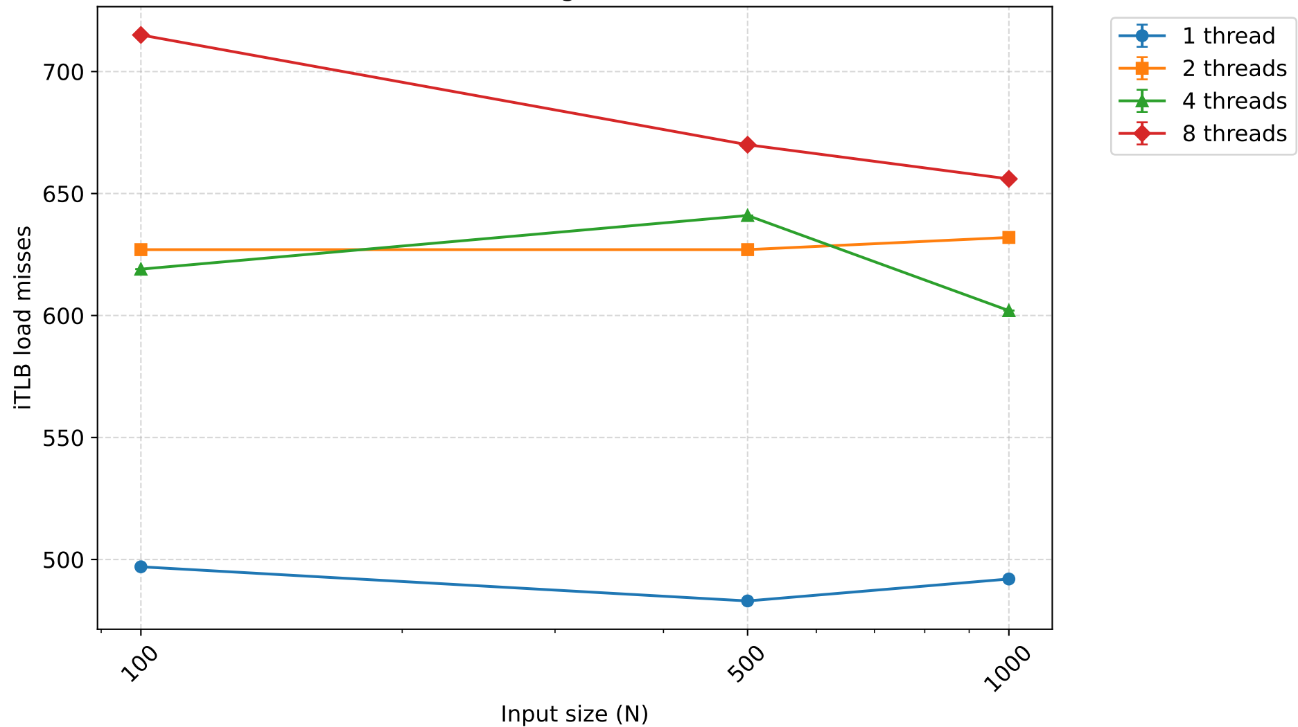
iTLB load misses - mergesort (mean \pm 95% CI)
