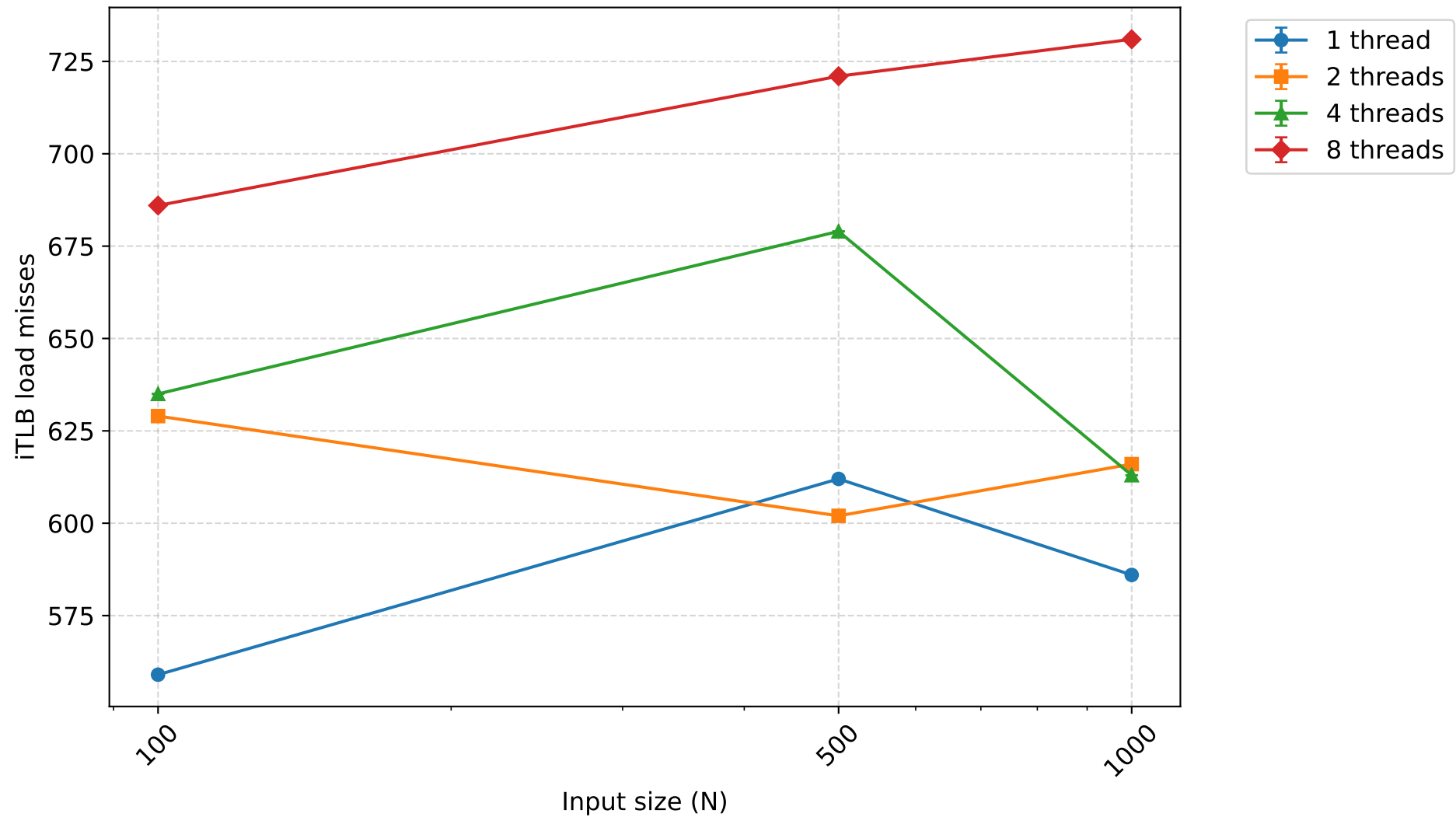
iTLB load misses - oddeven sort (mean \pm 95% CI)
