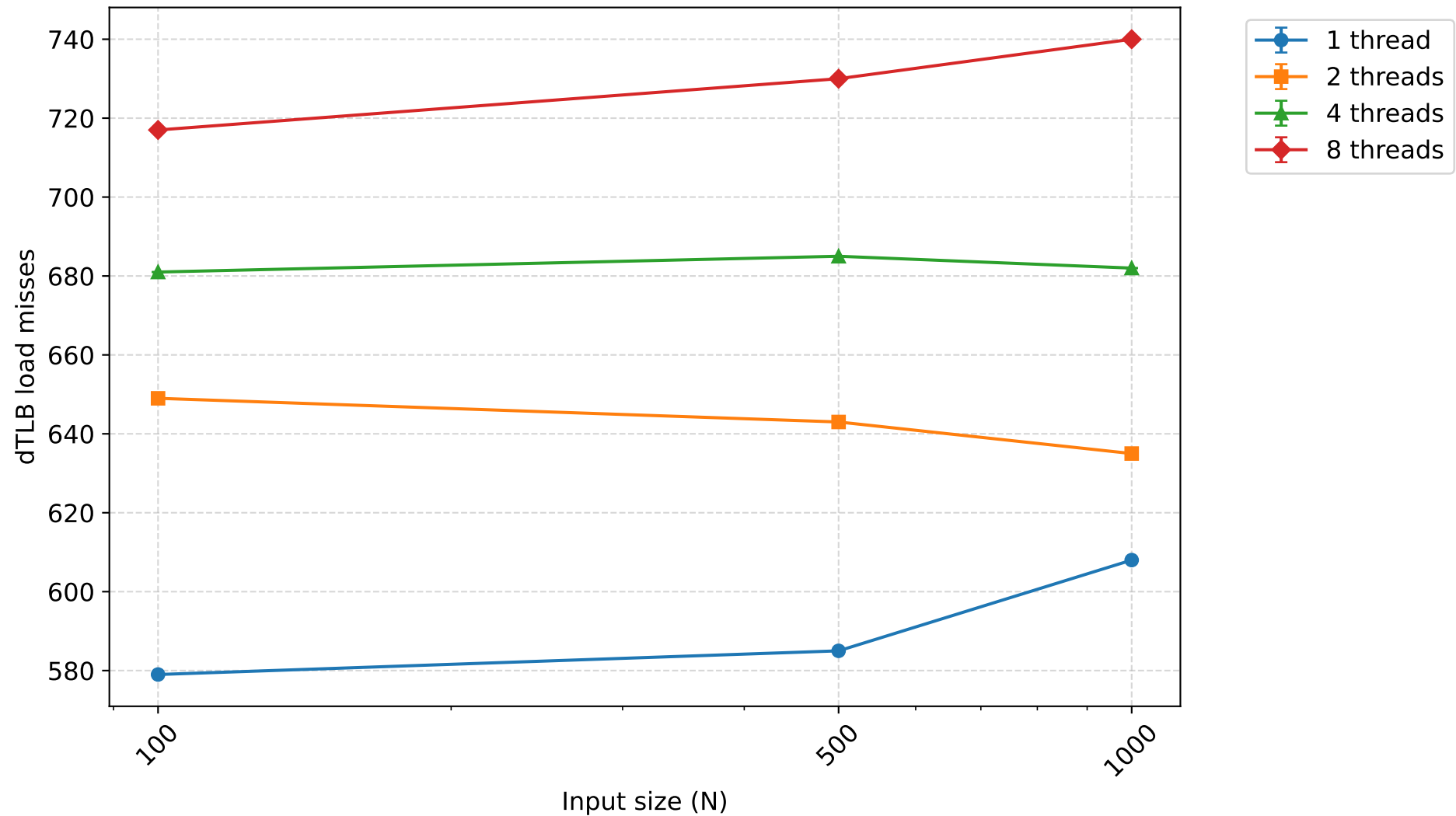
dTLB load misses - radixsort (mean \pm 95% CI)
