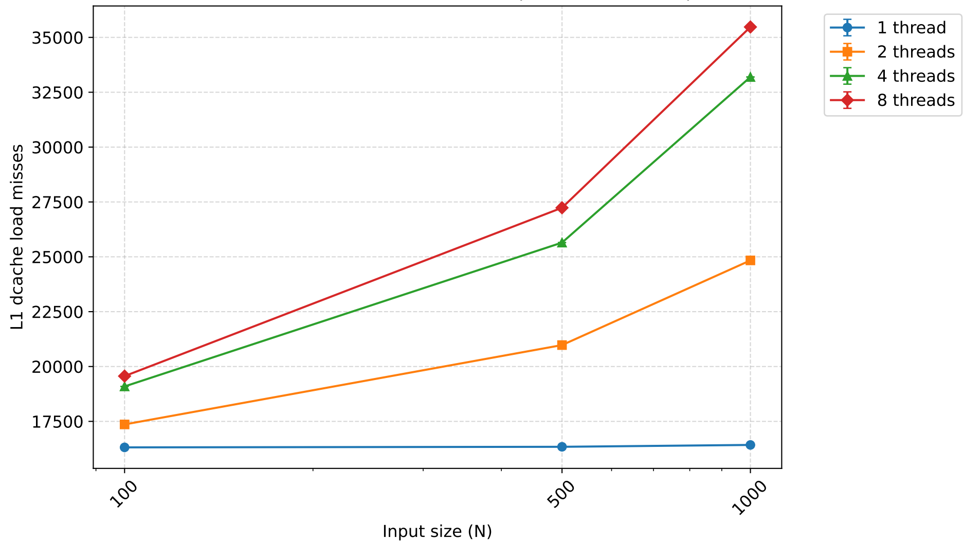
L1 dcache load misses - shellsort (mean \pm 95% CI)
