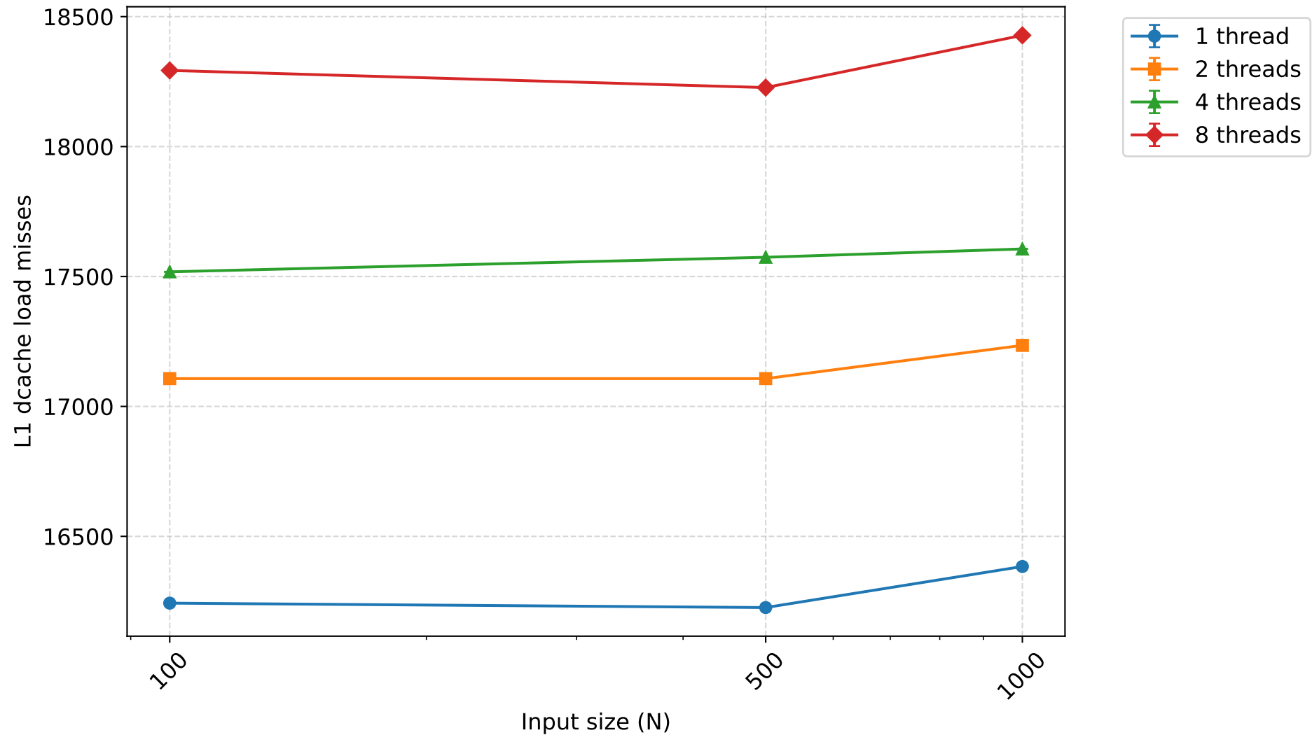
L1 dcache load misses - smoothsort (mean \pm 95% CI)
