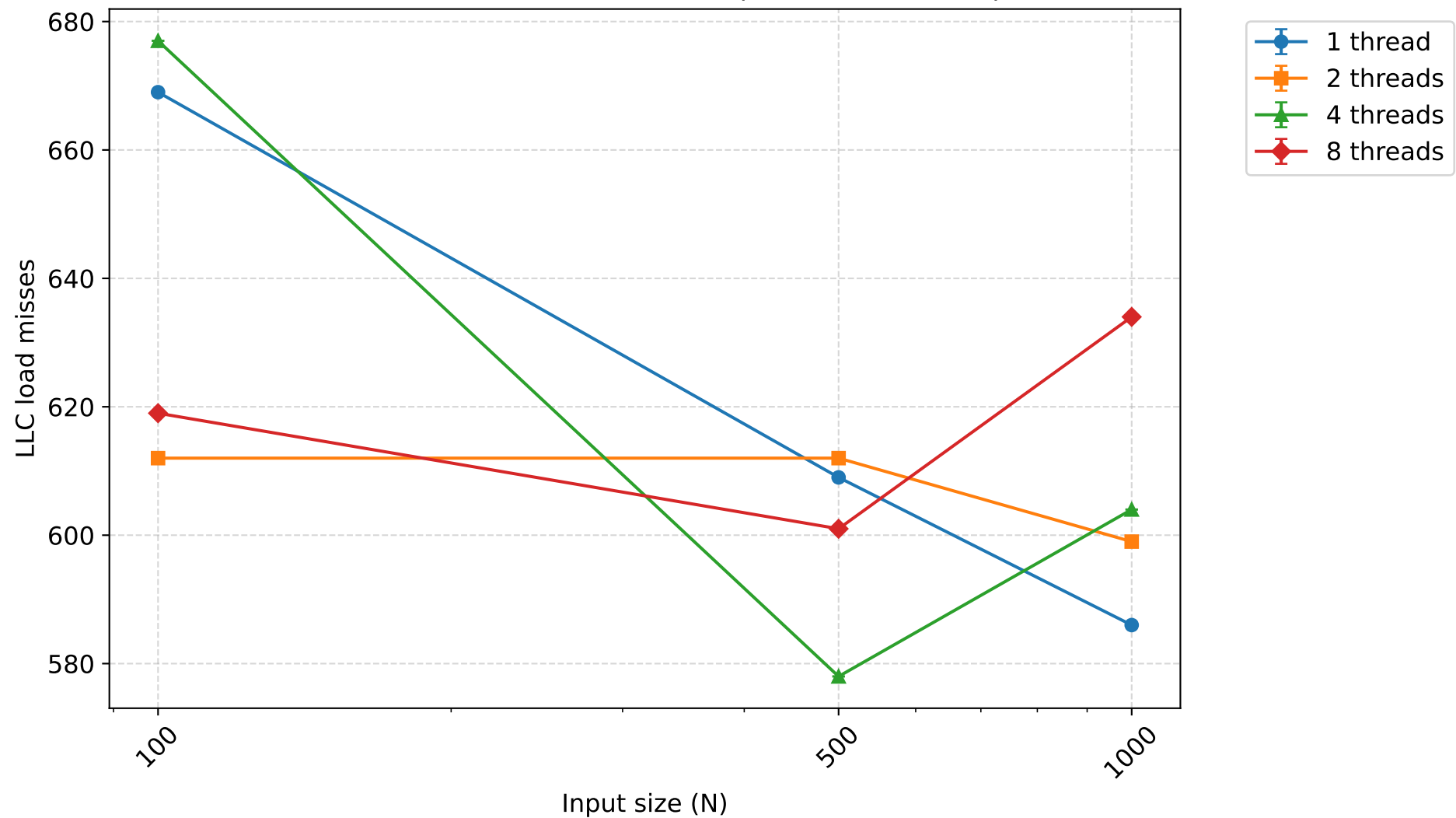
LLC load misses - smoothsort (mean \pm 95% CI)
