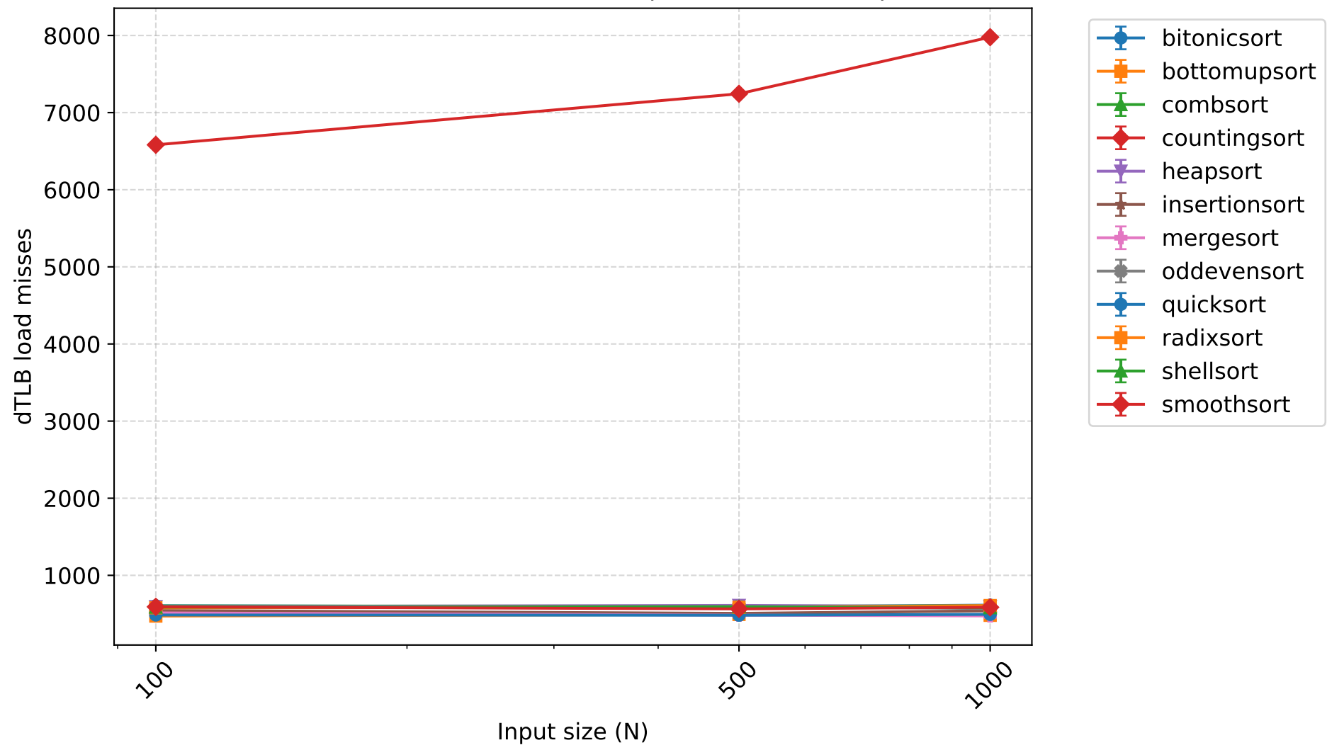
dTLB load misses - 1 thread (mean +- 95% CI)
