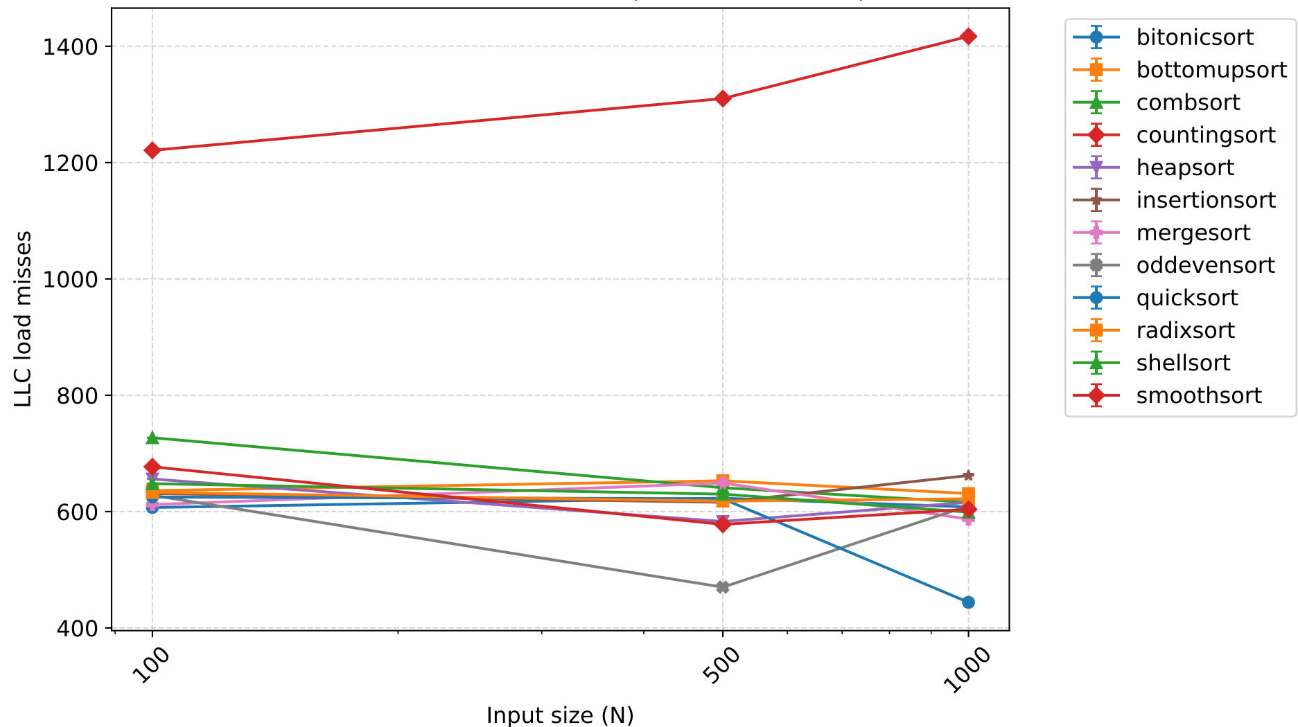
LLC load misses - 4 threads (mean \pm 95% CI)
