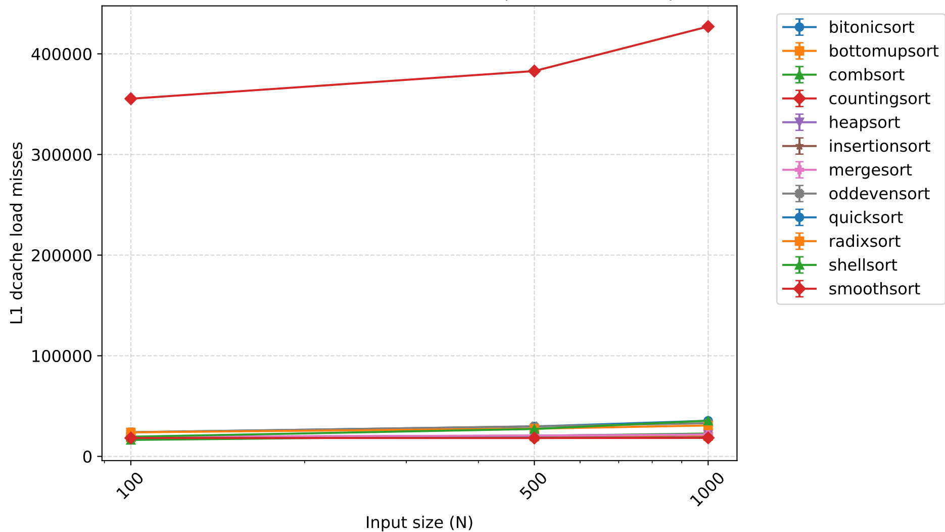
L1 dcache load misses - 8 threads (mean \pm 95% CI)
