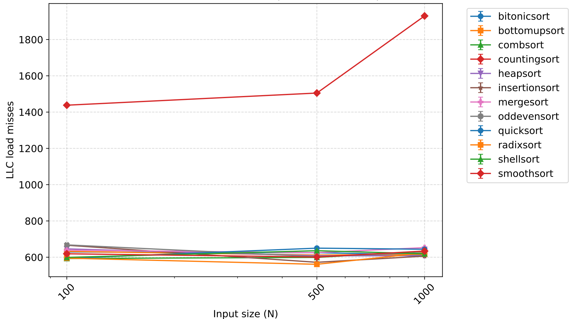
LLC load misses - 8 threads (mean \pm 95% CI)
