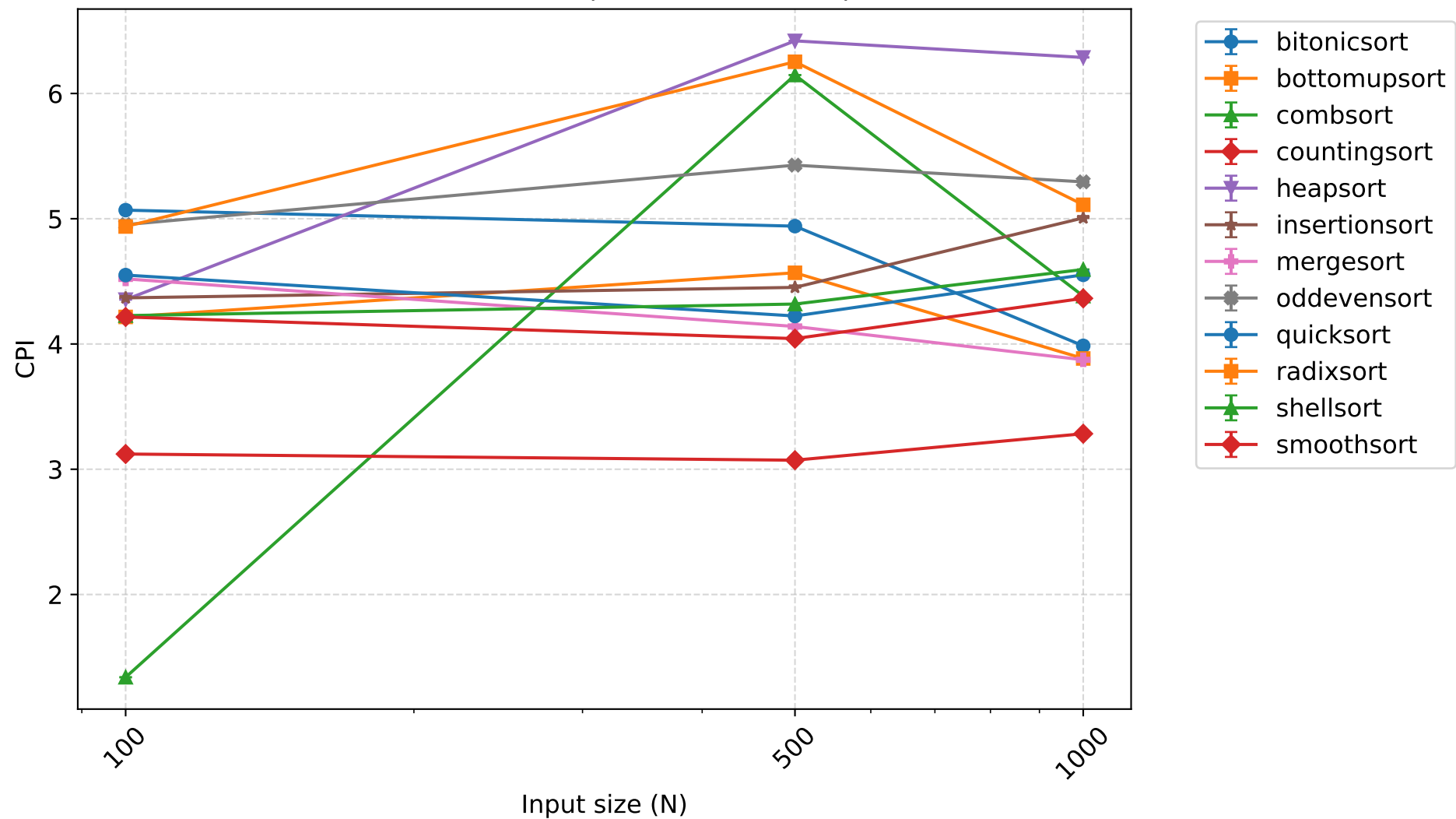
CPI - 8 threads (mean \pm 95% CI)
