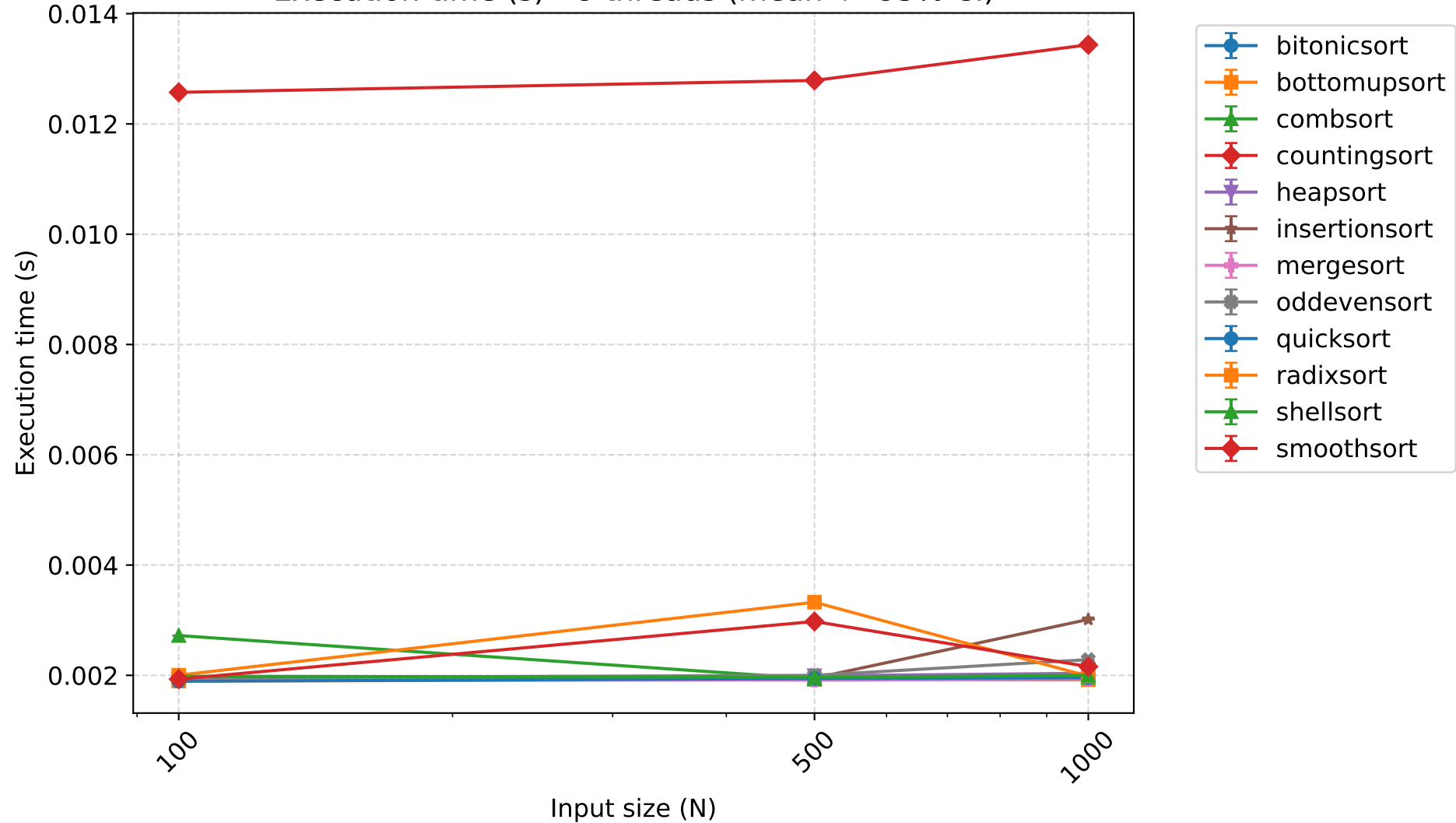
Execution time (s) - 8 threads (mean \pm 95% CI)
