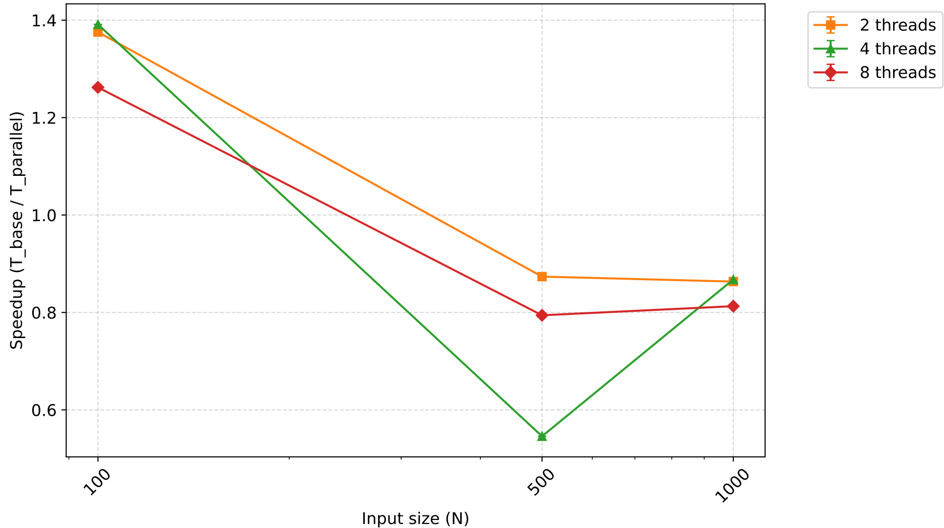
Speedup - bottomupsort (mean \pm 95% CI)
