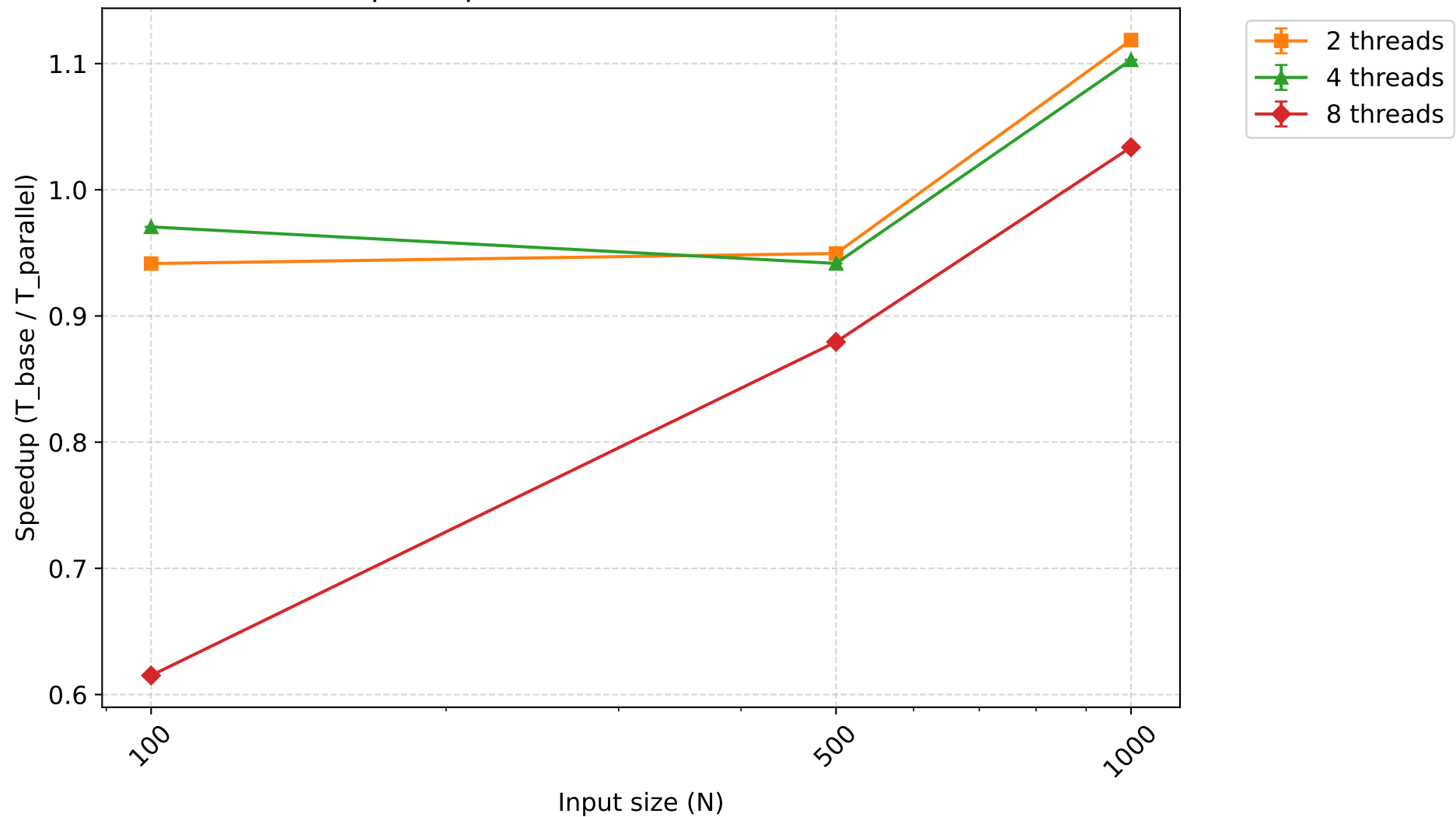
Speedup - combsort (mean \pm 95% CI)
