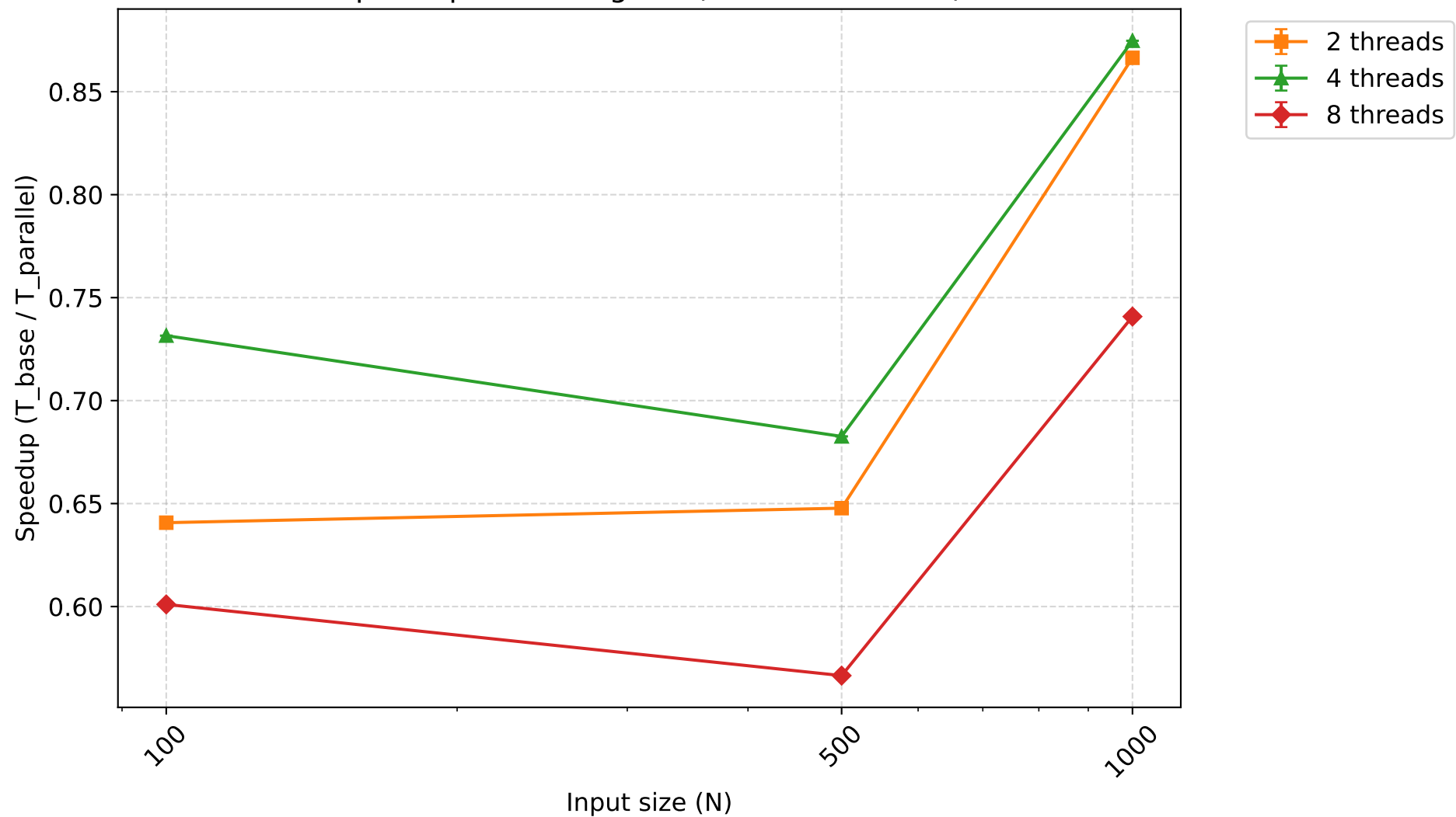
Speedup - countingsort (mean \pm 95% CI)
