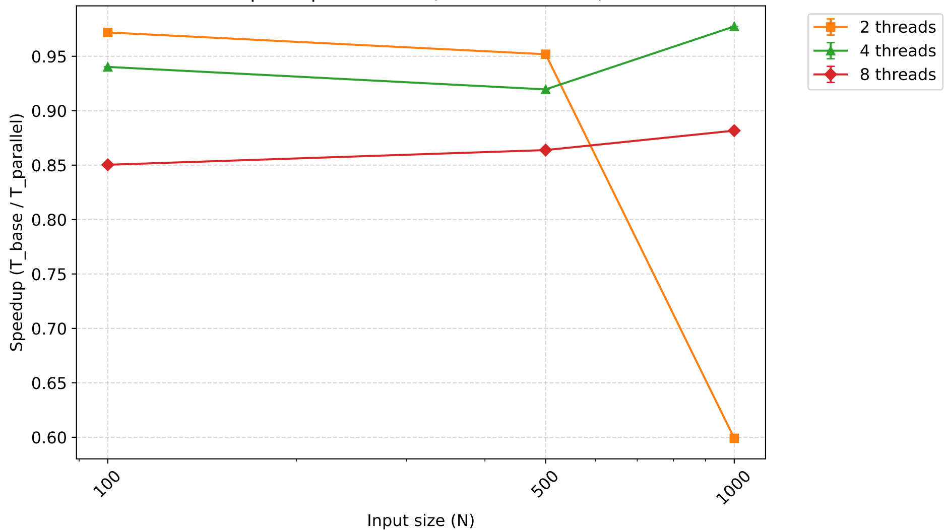
Speedup - shellsort (mean \pm 95% CI)
