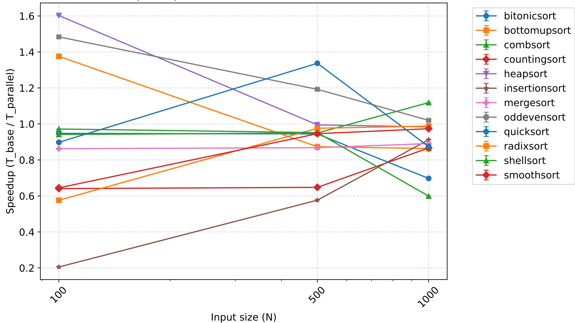
Speedup - 2 threads (mean \pm 95% CI)
