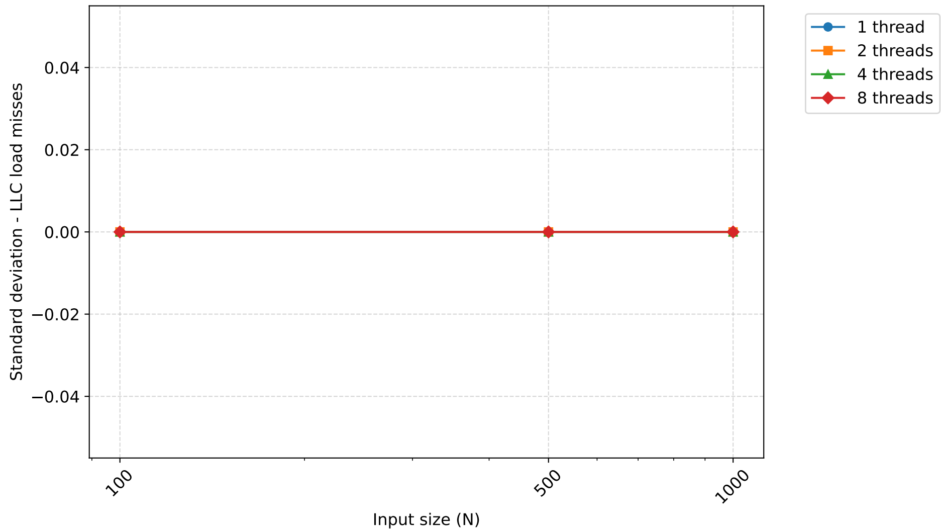
Standard deviation of LLC load misses - radixsort
