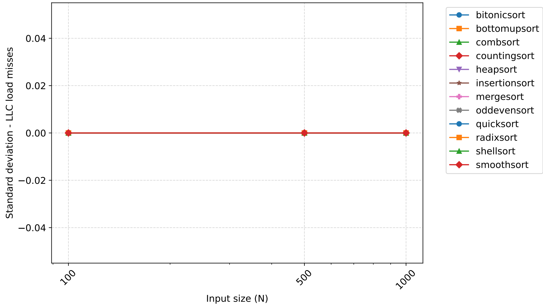
Standard deviation of LLC load misses - 4 threads
