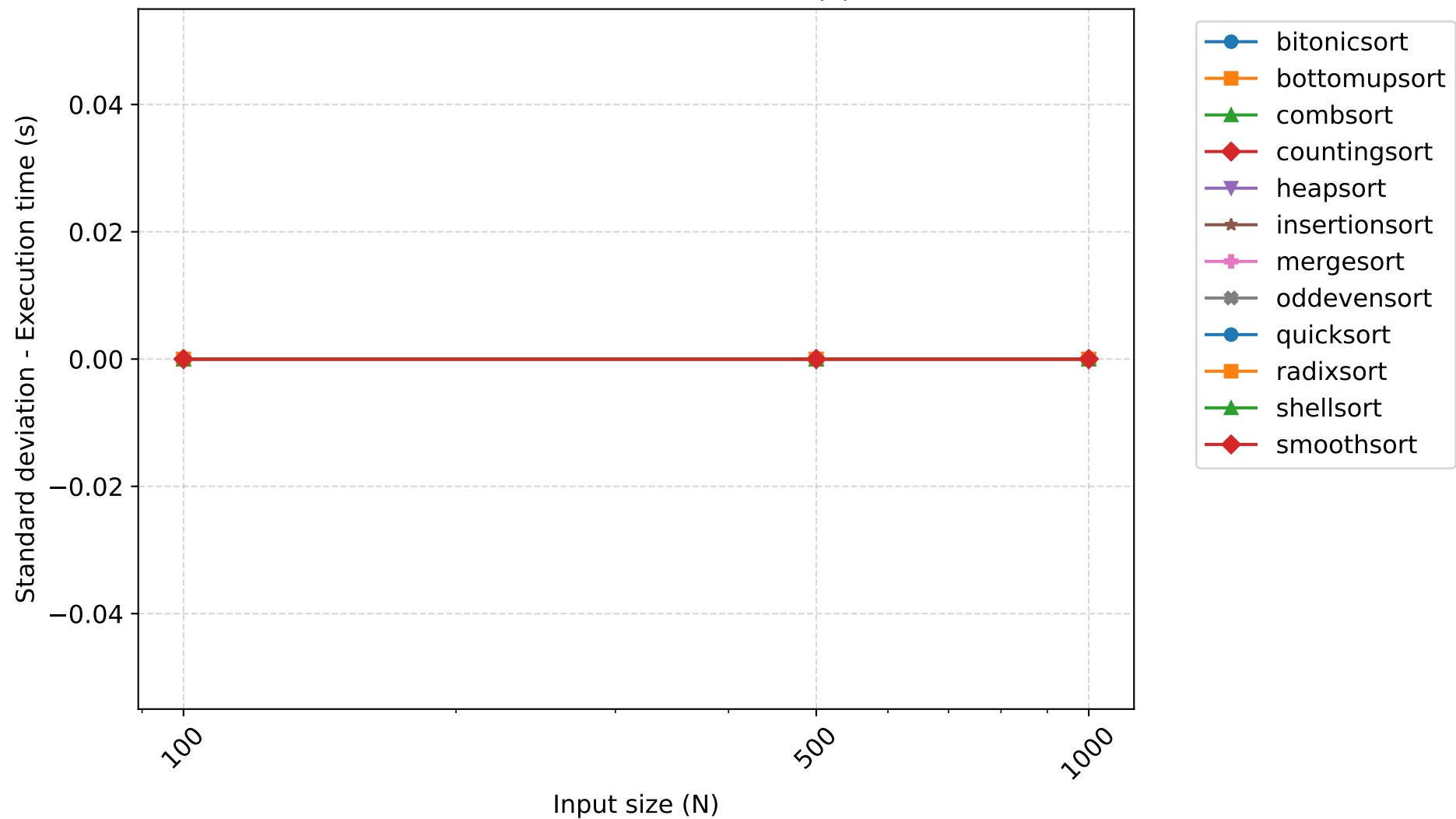
Standard deviation of Execution time (s) - 8 threads
