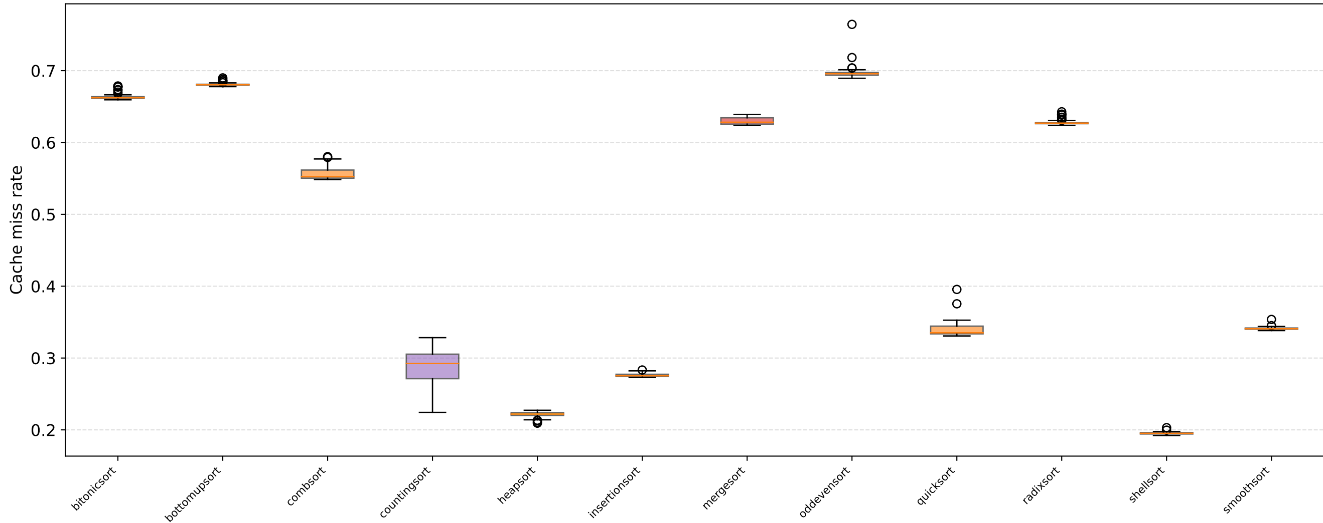
Distribution over repetitions (N=10000000, serial)
