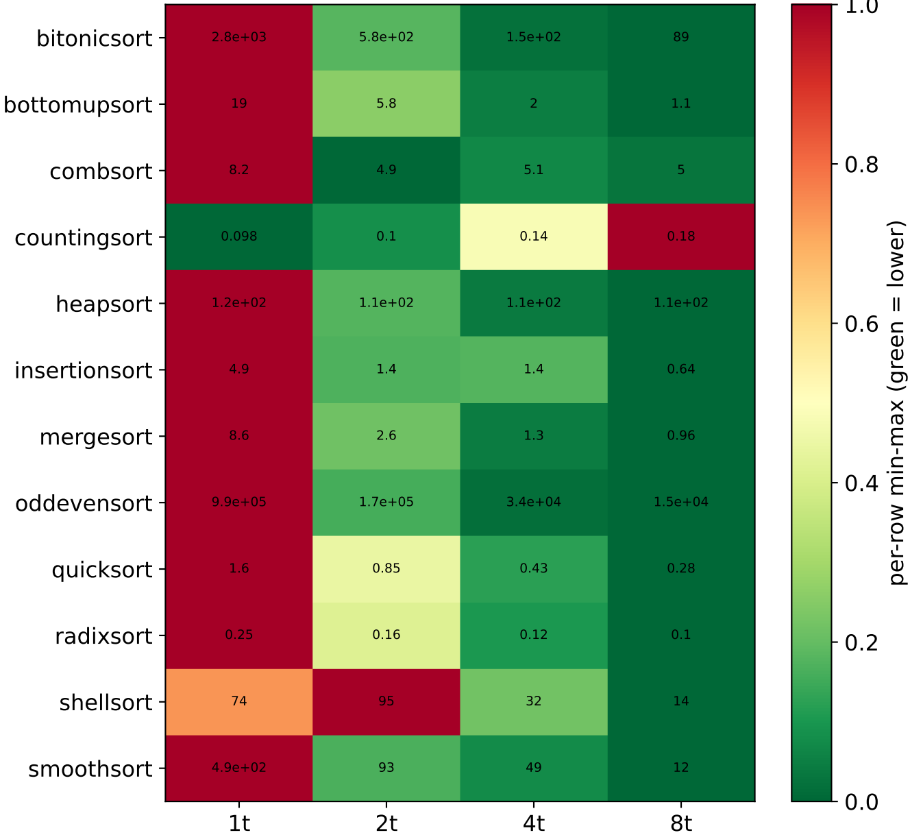
ED 2 P (J·s 2 ) by algorithm × threads (N=10000000) — green = best per row
