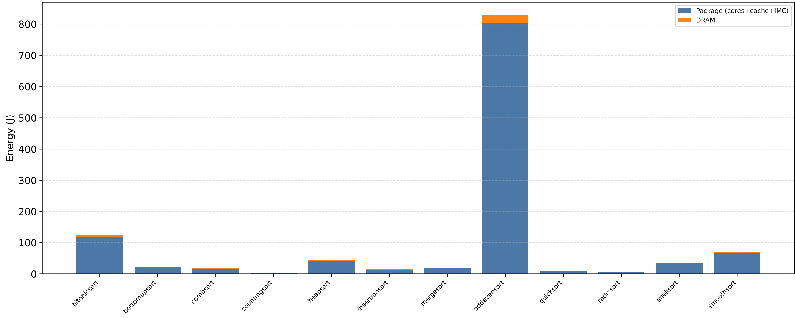
Energy breakdown: package vs DRAM (N=10000000, serial)
