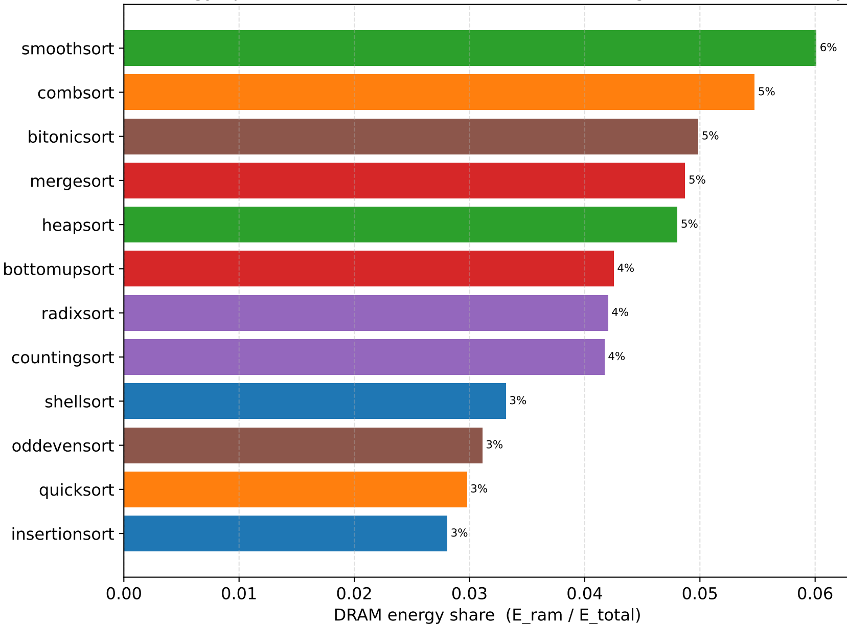
Share of energy spent in DRAM (N=10000000, serial) — higher = more memory-bound
