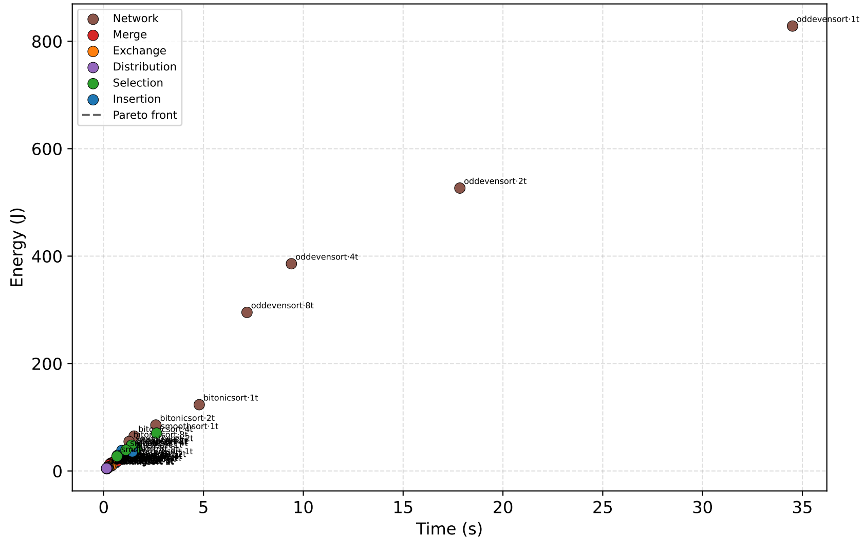
Energy-time trade-off (N=10000000, all thread counts)
