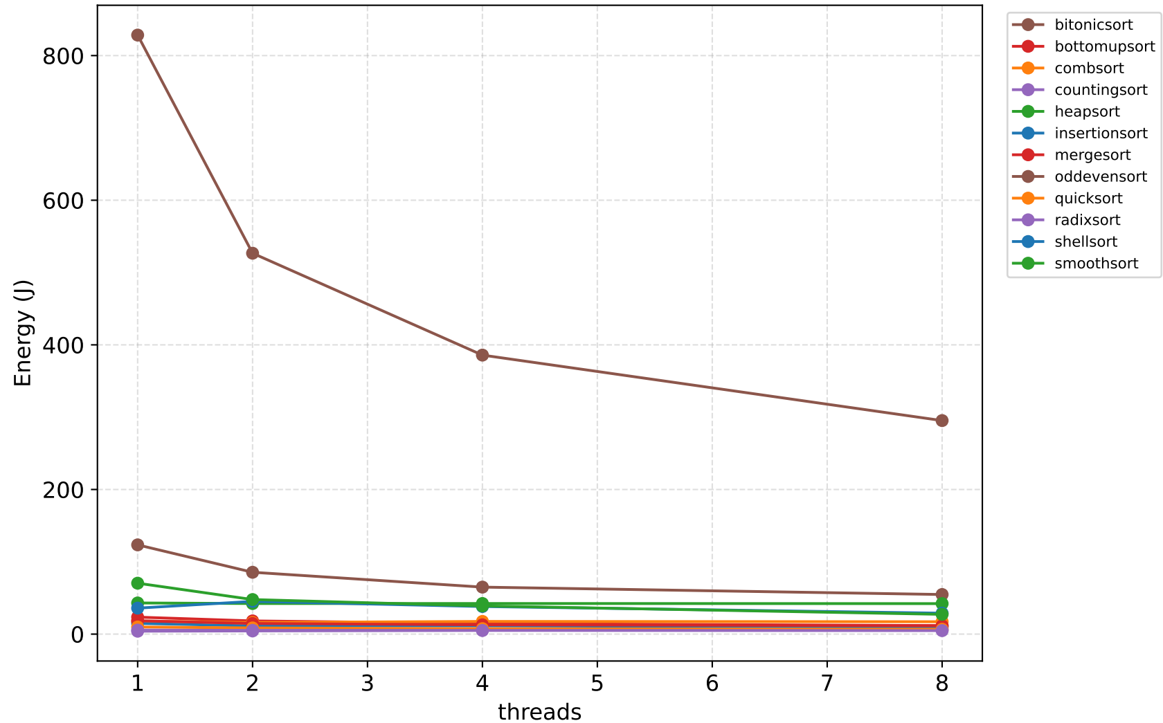
Total energy vs threads (N=100000000) — does not drop like time
