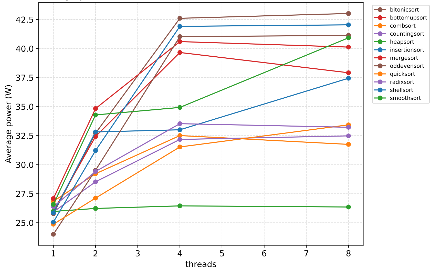
Average power vs threads (N=10000000) — rises with active cores
