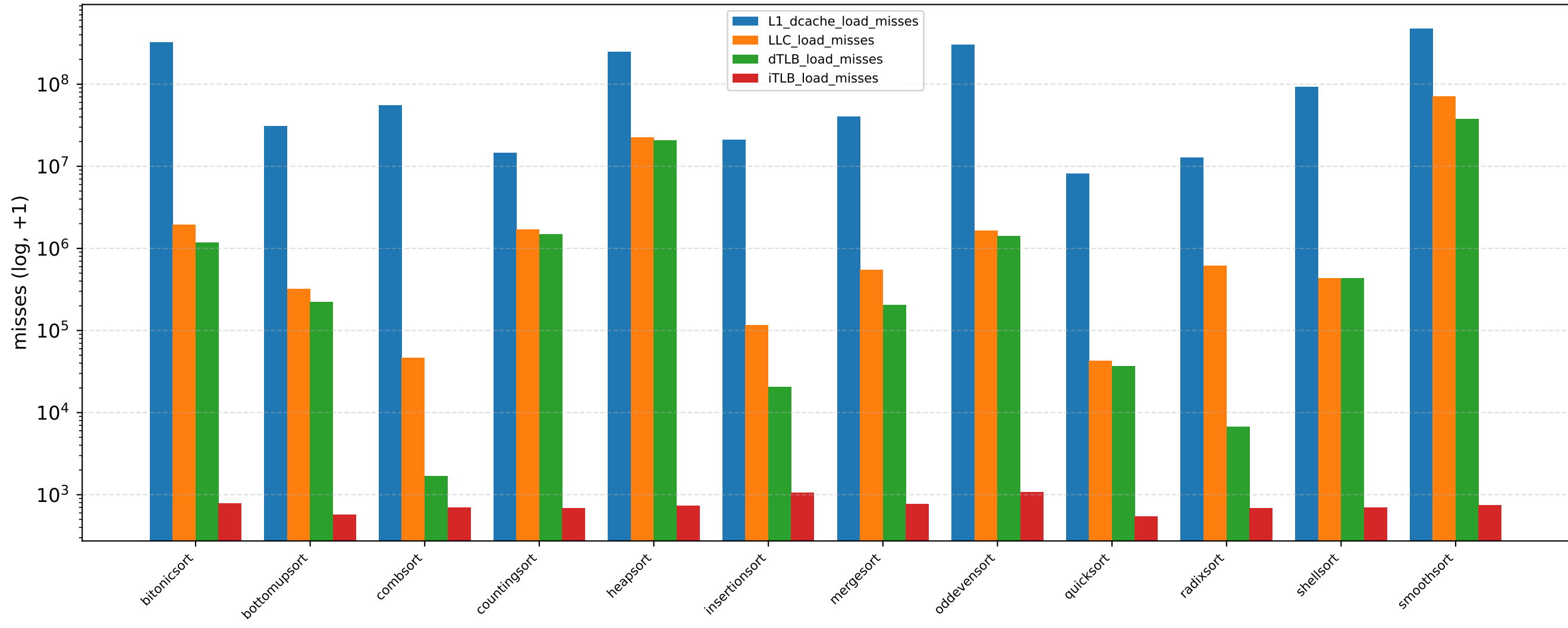
Memory hierarchy pressure (N=10000000, serial)
