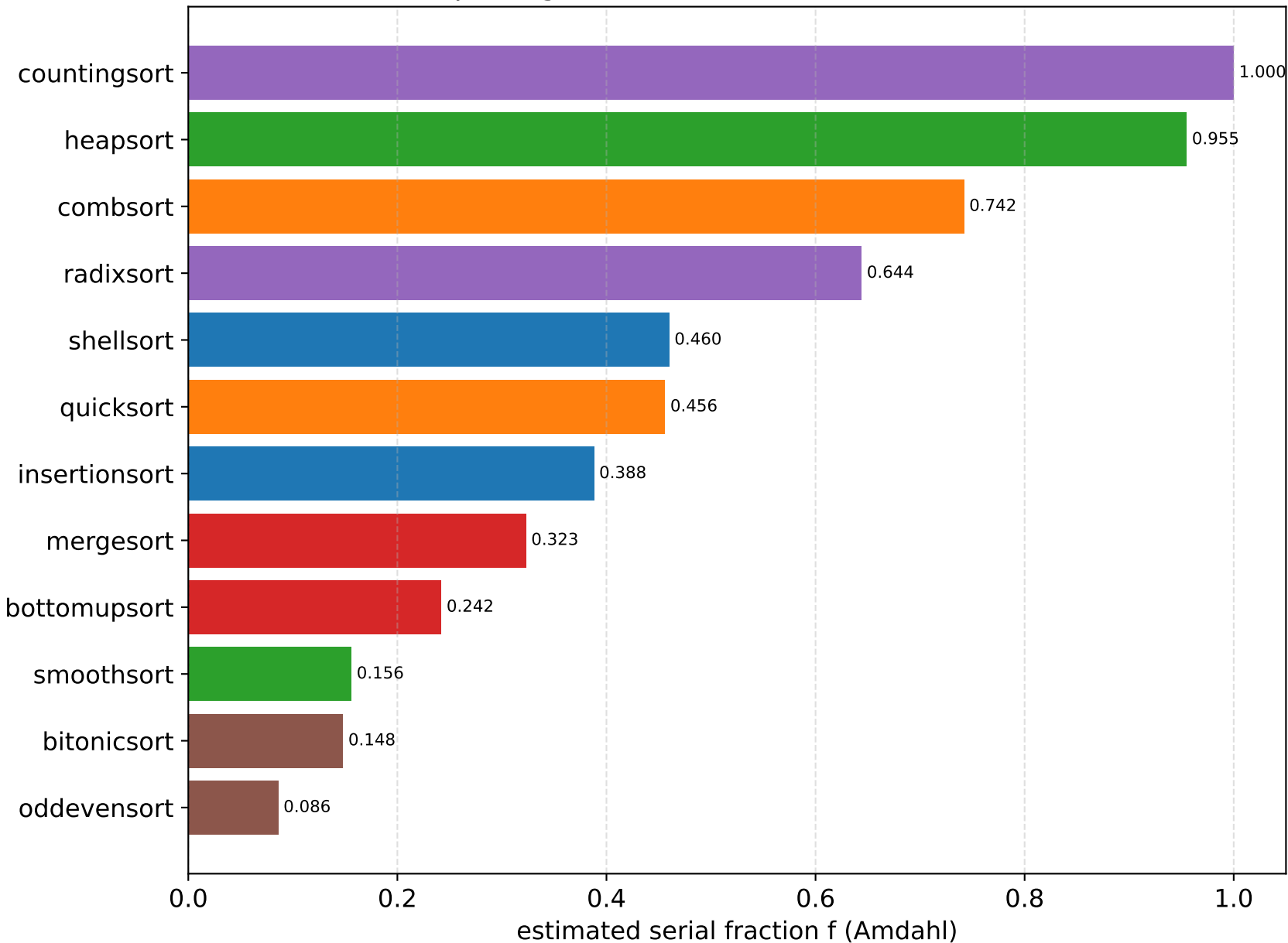
Serial fraction per algorithm (N=10000000) — lower f scales better
