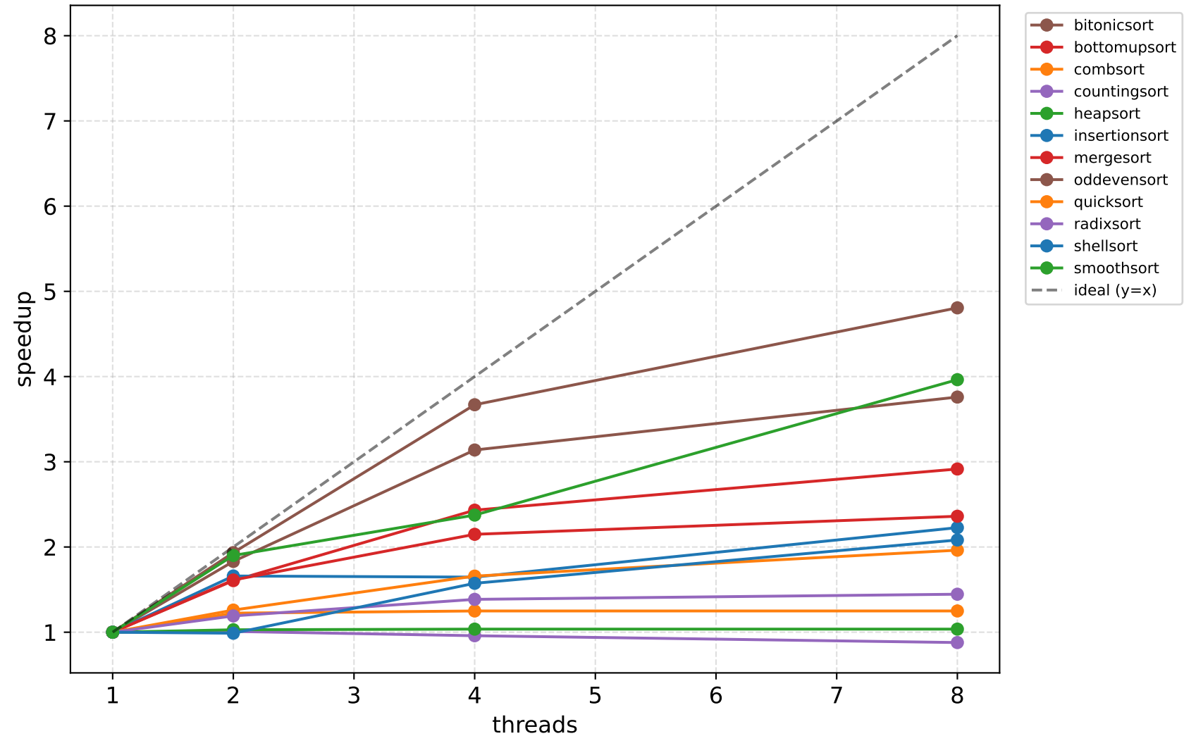
Speedup vs threads (N=10000000) with ideal line
