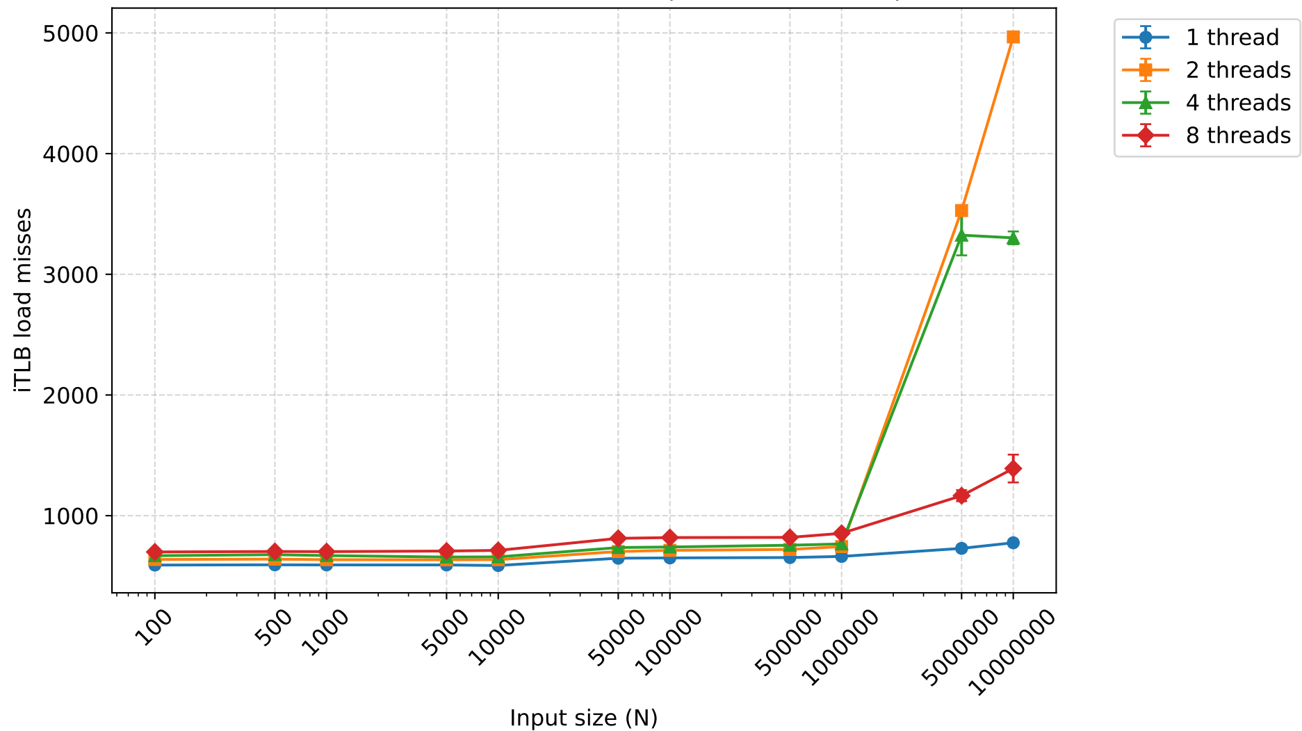
iTLB load misses - bitonicsort (mean \pm 95% CI)
