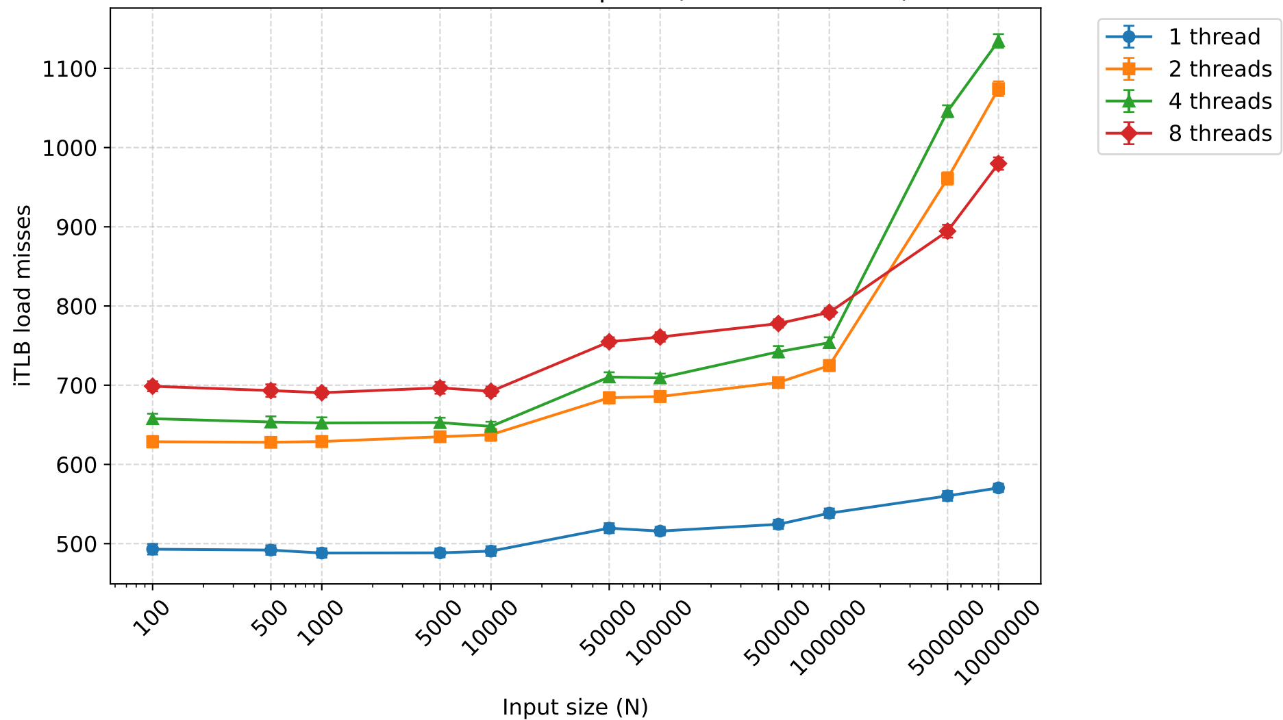
iTLB load misses - bottomupsort (mean \pm 95% CI)
