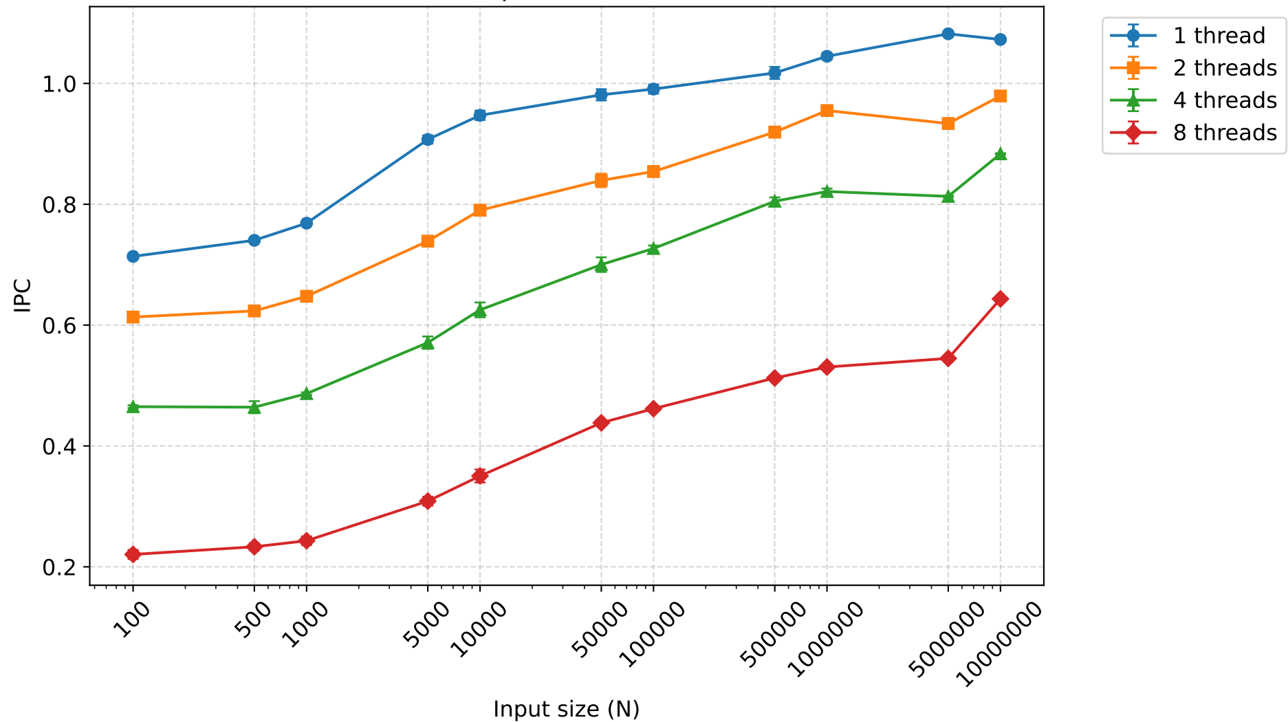
IPC - bottomupsort (mean \pm 95% CI)
