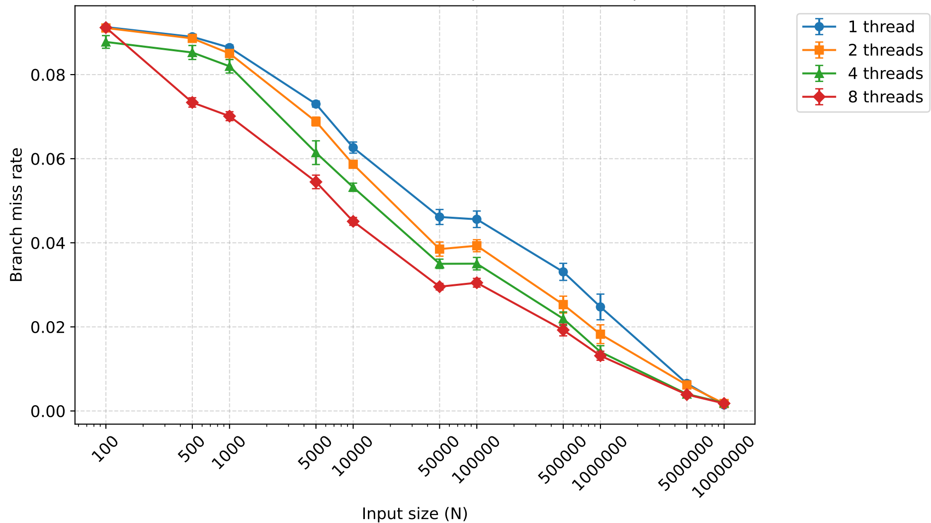
Branch miss rate - combort (mean \pm 95% CI)
