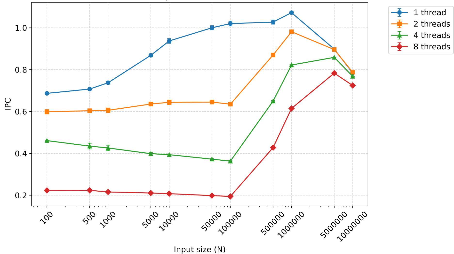
IPC - heapsort (mean \pm 95% CI)
