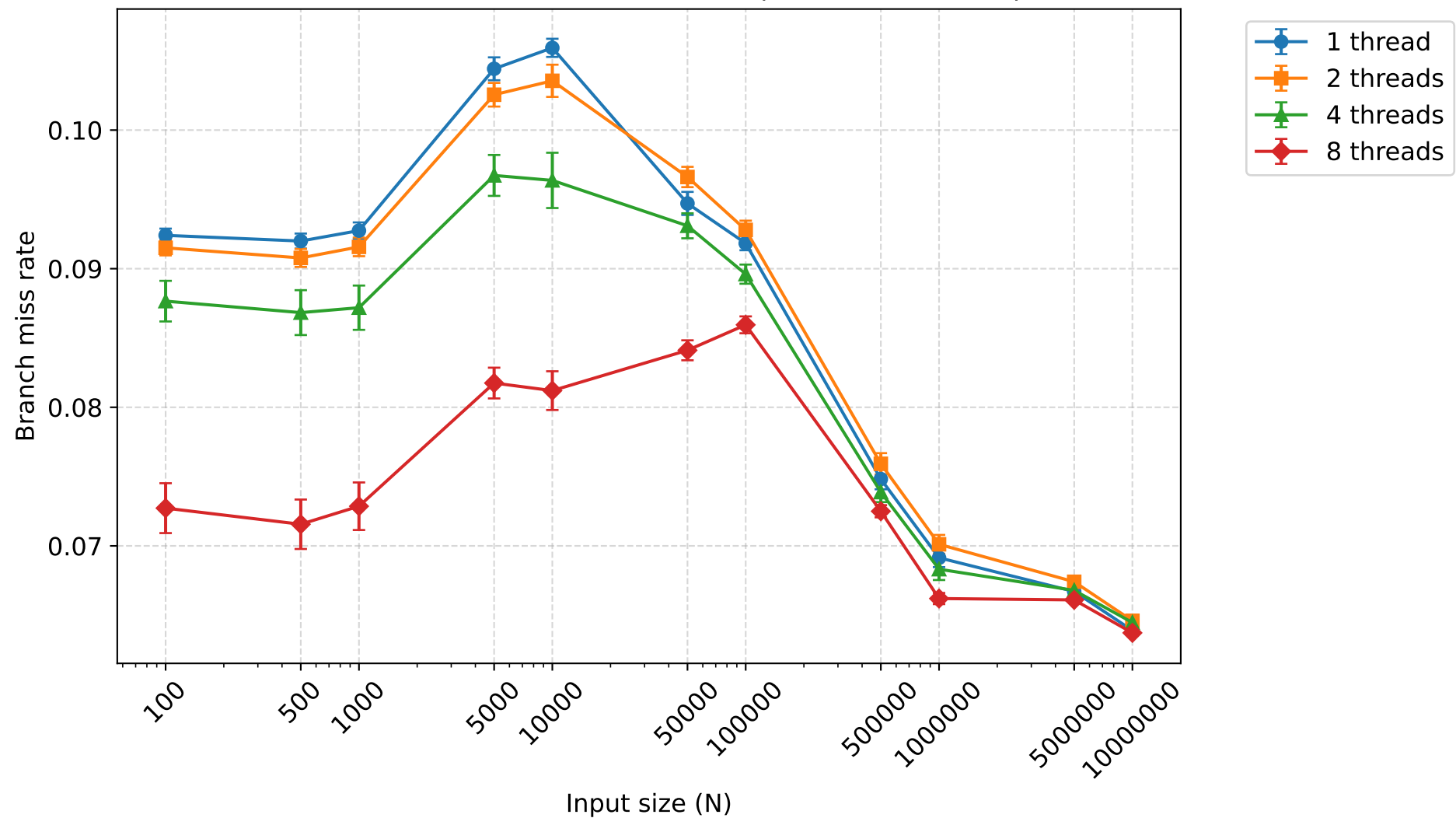
Branch miss rate - insertionsort (mean \pm 95% CI)
