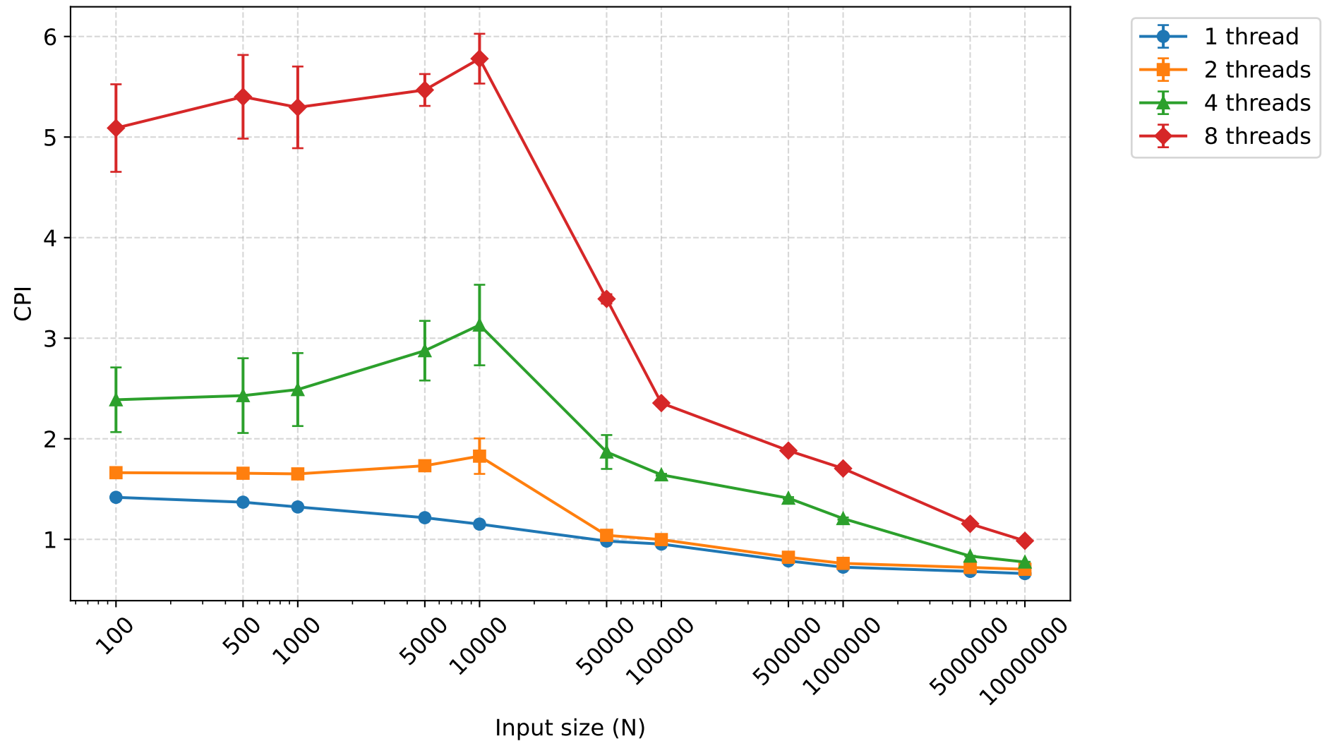
CPI - insertionsort (mean \pm 95% CI)
