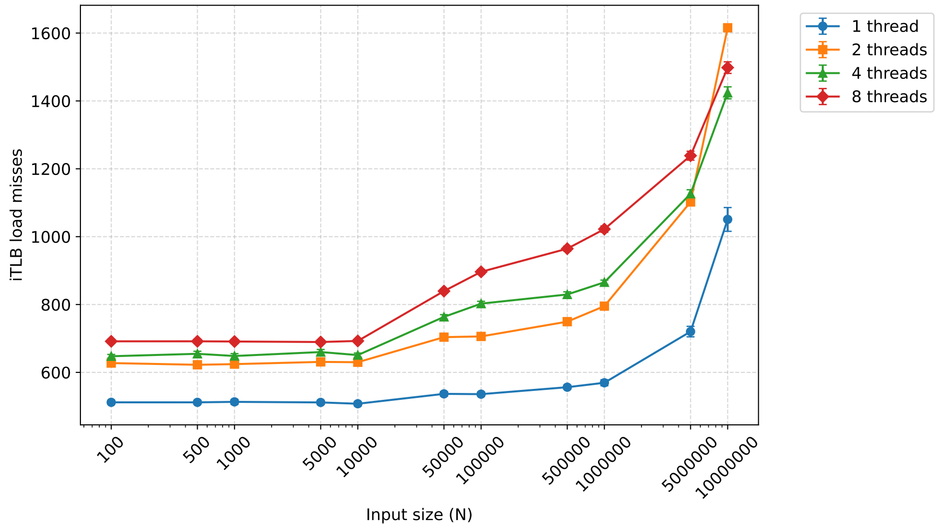
iTLB load misses - insertionsort (mean \pm 95% CI)
