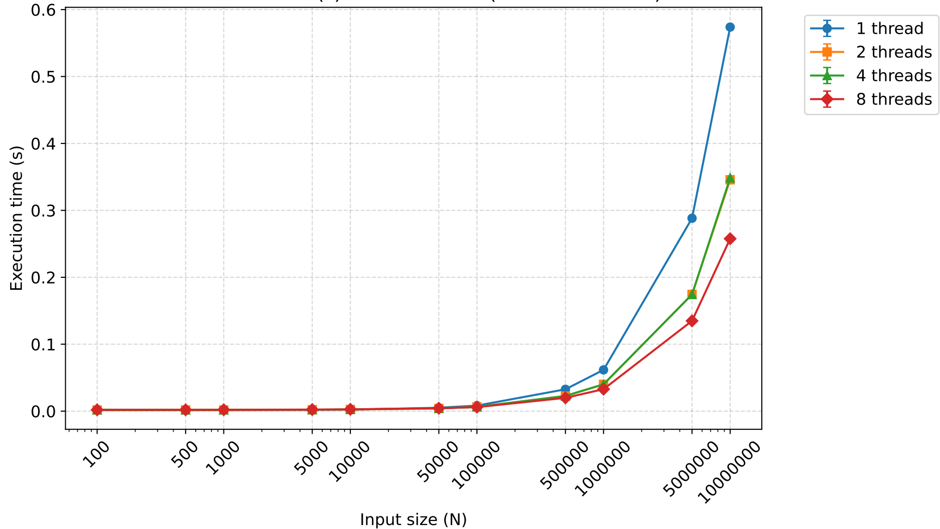
Execution time (s) - insertion sort (mean \pm 95% CI)
