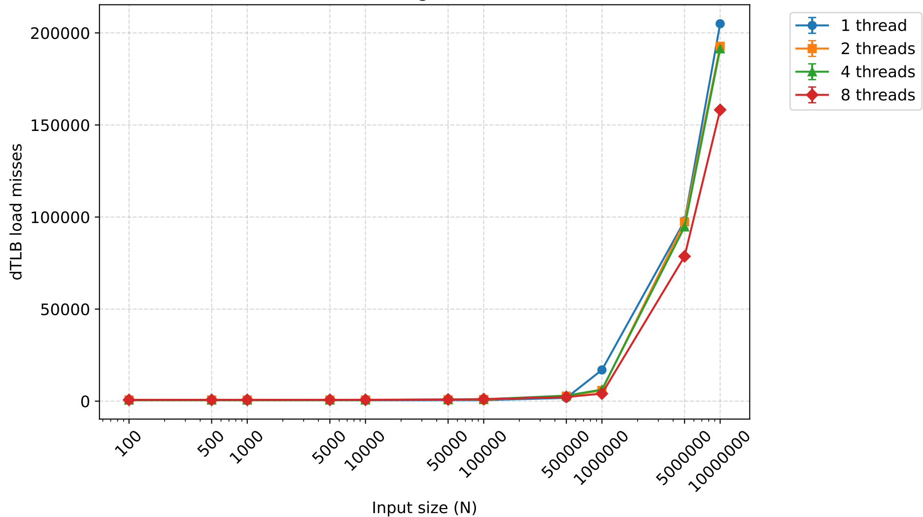
dTLB load misses - mergesort (mean \pm 95% CI)
