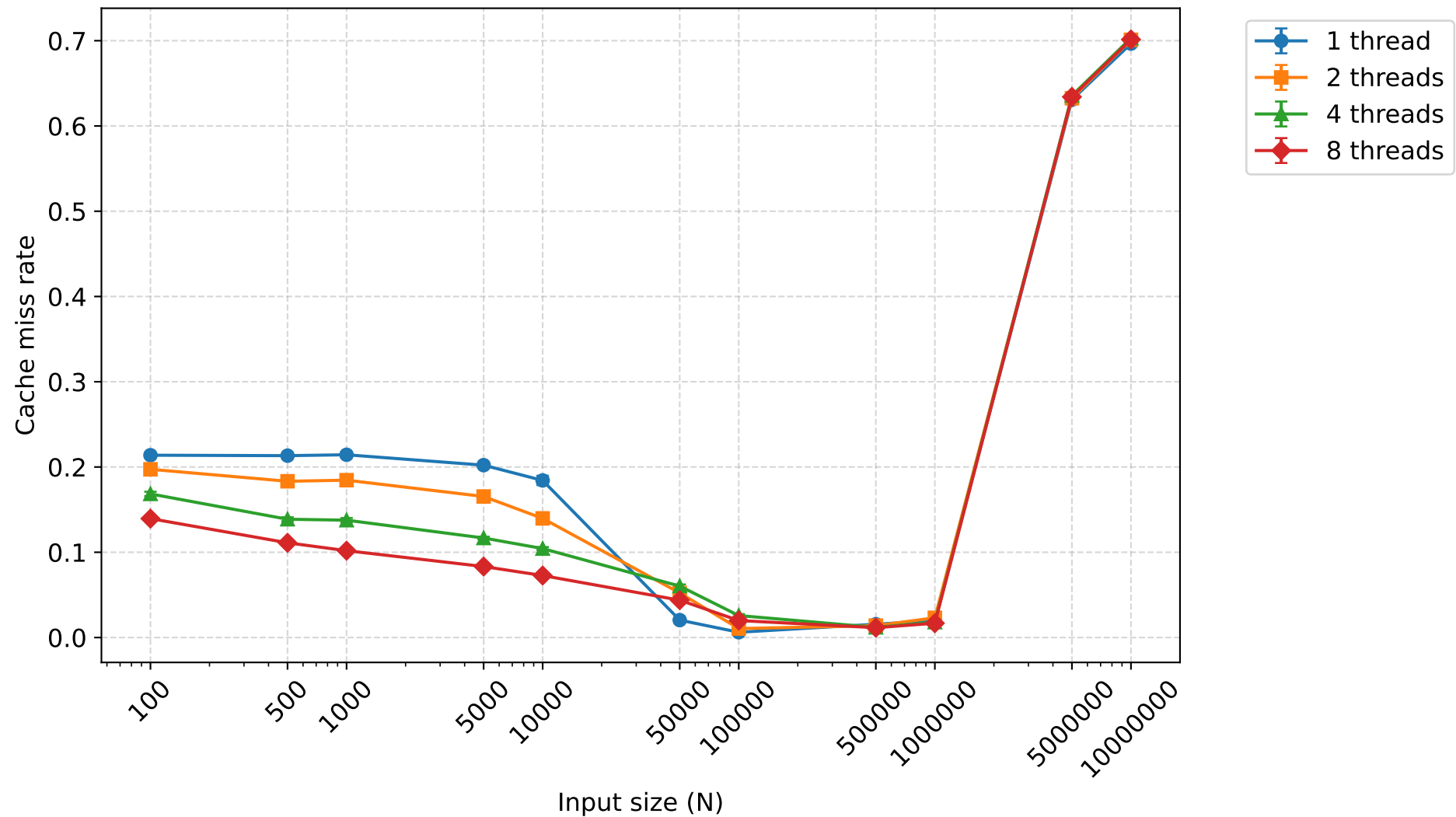
Cache miss rate - oddevensort (mean \pm 95% CI)
