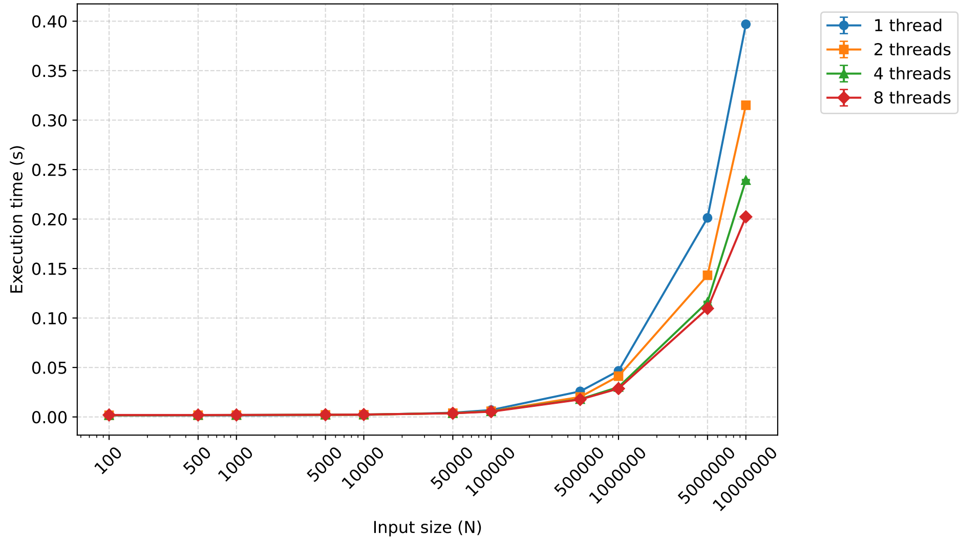
Execution time (s) - quicksort (mean \pm 95% CI)
