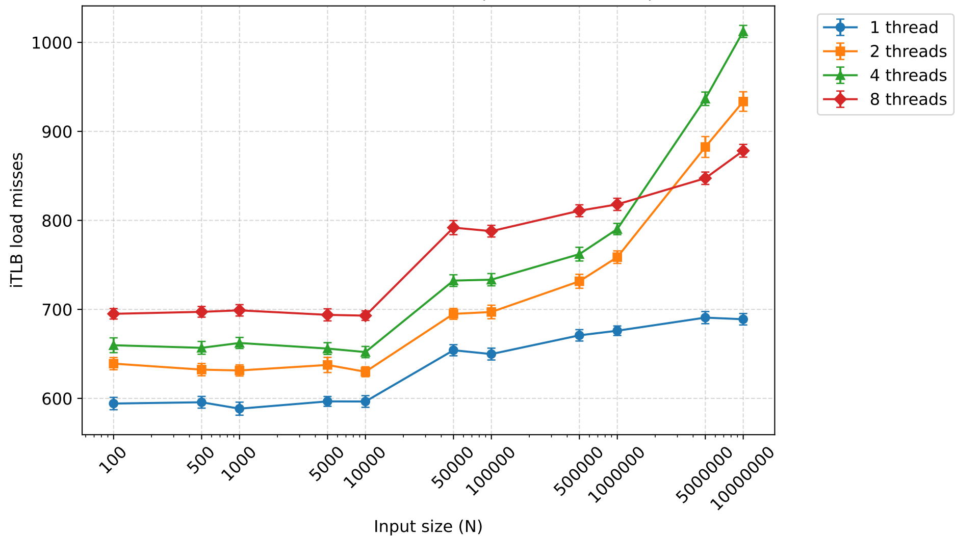
iTLB load misses - radixsort (mean \pm 95% CI)
